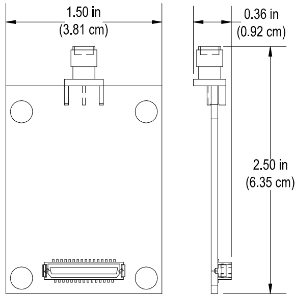
MNET-CWD1012 Detail Views
