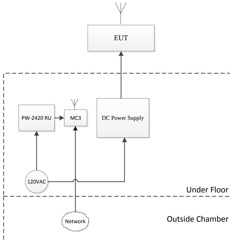
Test Setup Block Diagram
