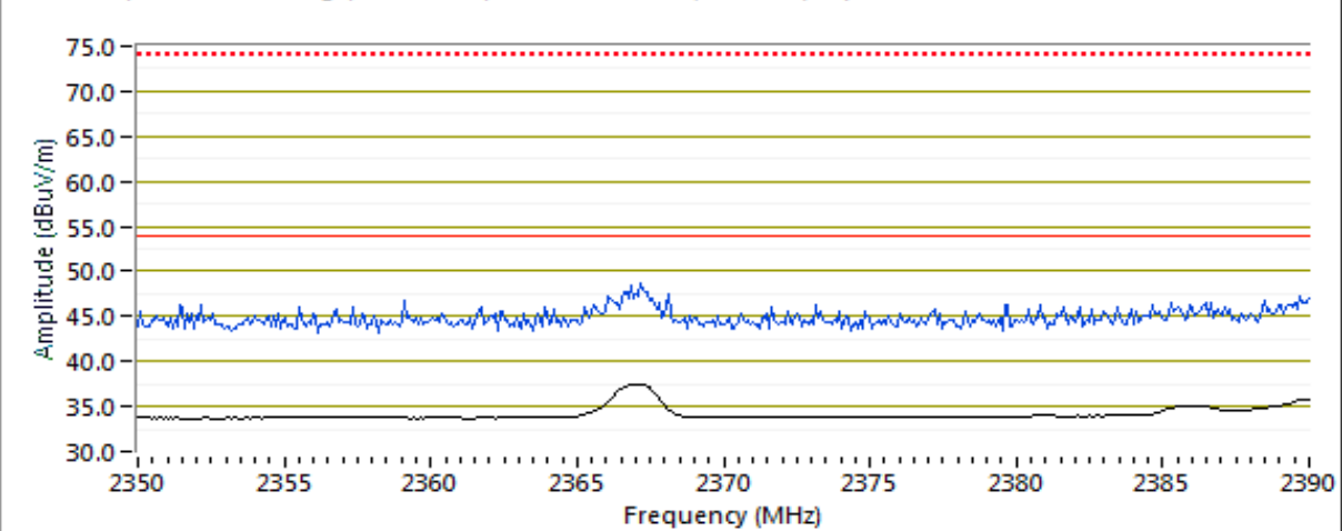
RB 1 MHz; VB 10 Hz Average, RB: 1 MHz; VB: 3 MHz Peak (Blue line) V-pol
