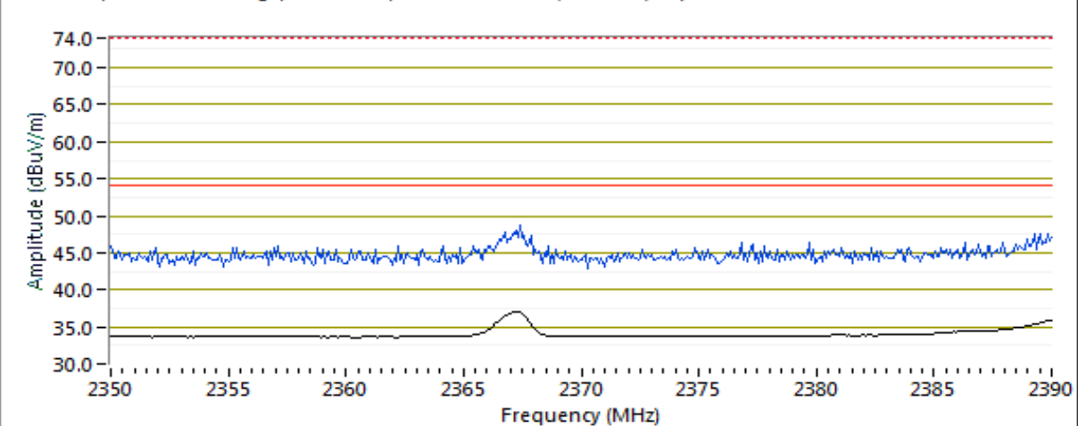
RB 1 MHz; VB 10 Hz Average, RB: 1 MHz; VB: 3 MHz Peak (Blue line) H-pol
