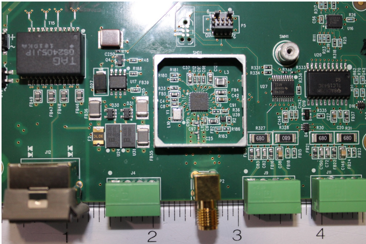
CLOSEUP OF RF – NO COVER
