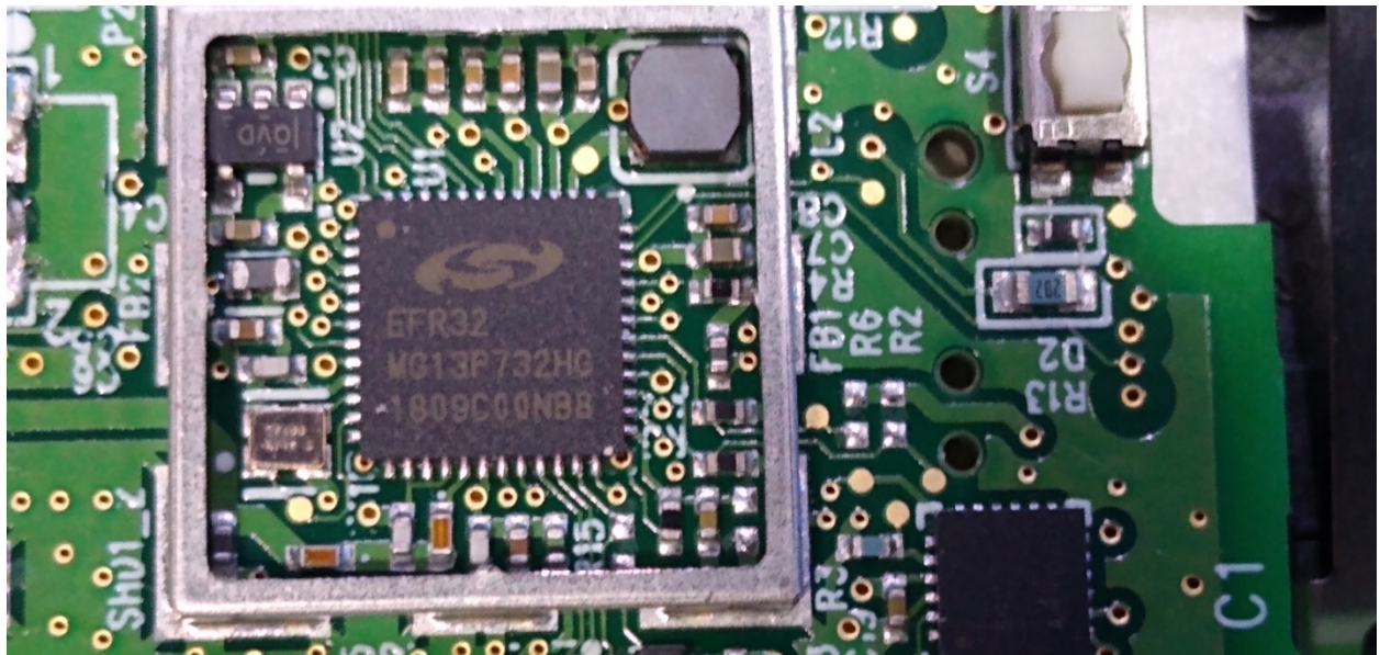
SHIELD REMOVED
