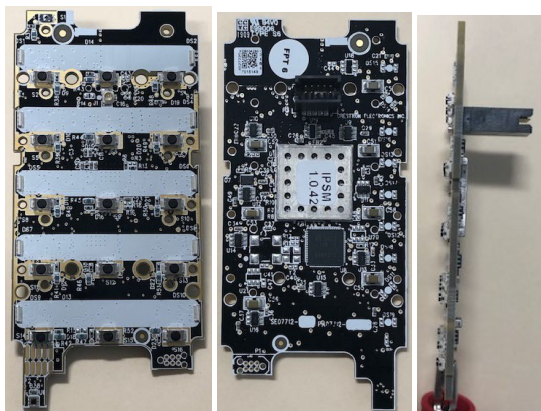
Physical View of CWD7969 (Front, Rear, Side)
