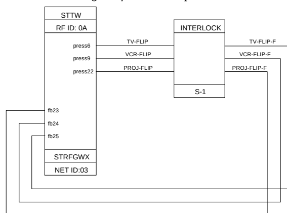
SIMPL Block Diagram for the Example
