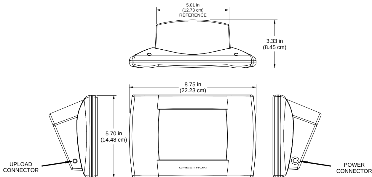
Physical Views of STX-1550C
