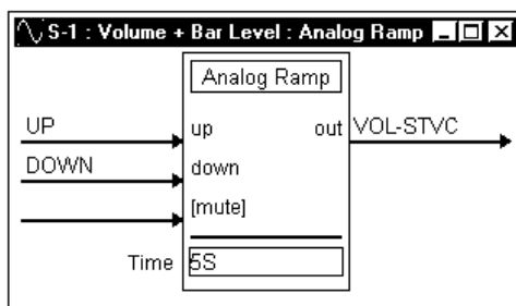
Detail View of an Analog Ramp (S-1) in SIMPL Windows' Programming Manager
