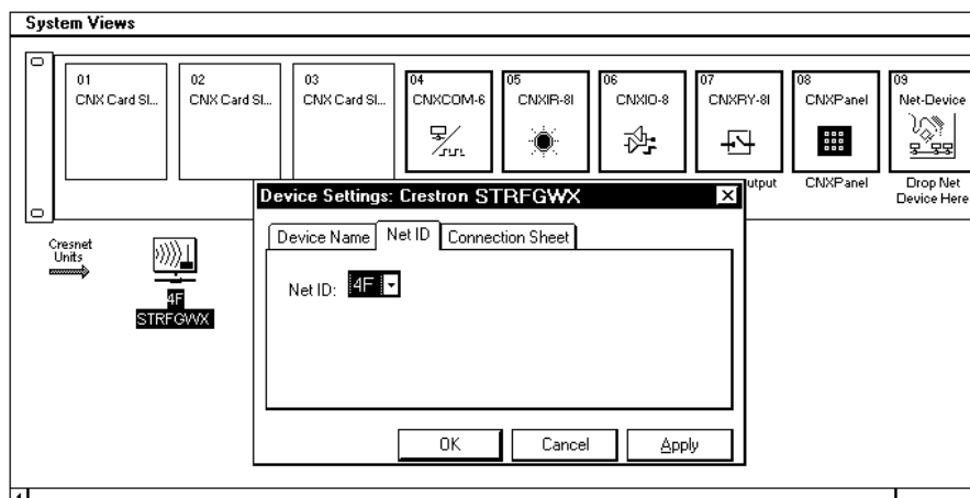
System View of STRFGWX NET ID Assignment in SIMPL Windows' Configuration Manager
