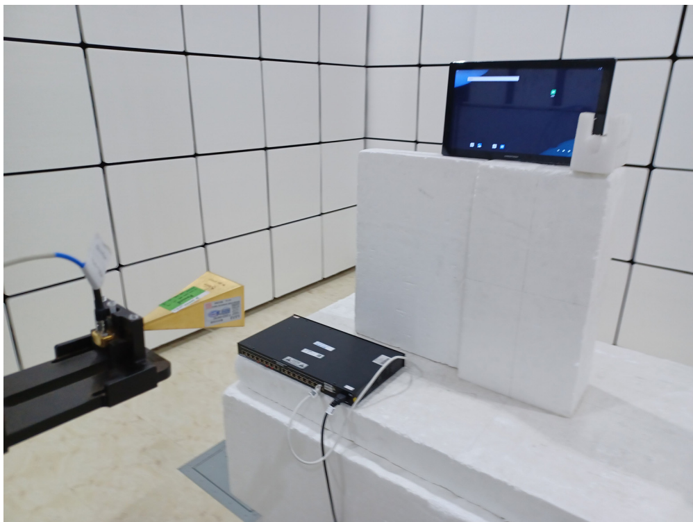
Radiated Test (Above 40 GHz)
