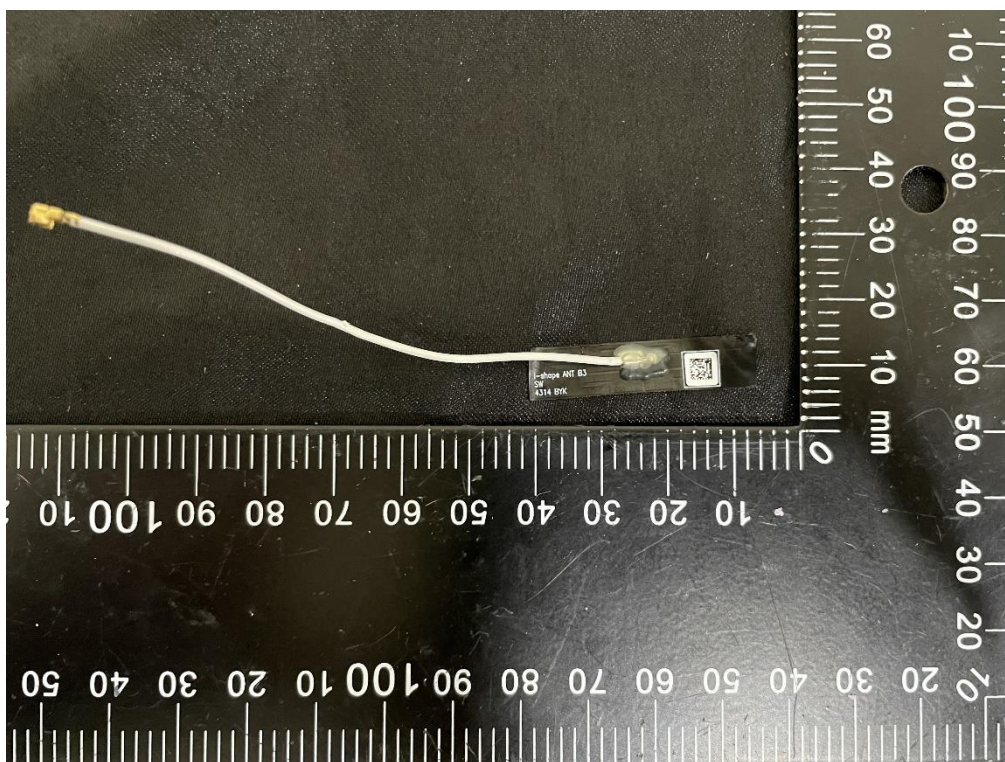
Main Antenna
