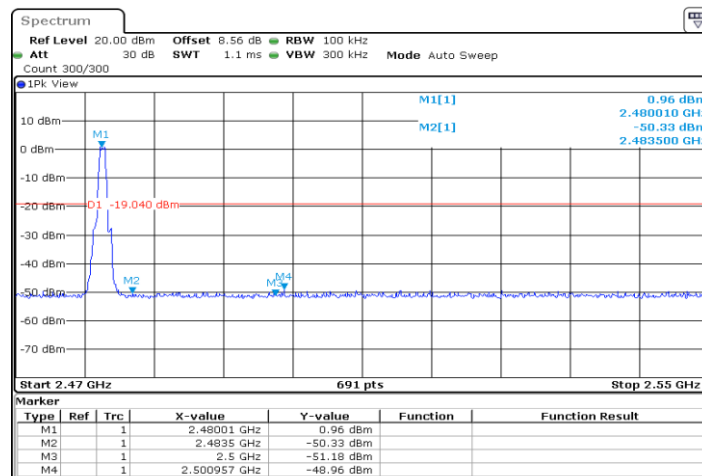
LE 1M_Ant1_High_2480
