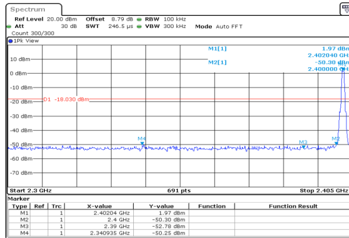
LE 1M_Ant1_Low_2402
