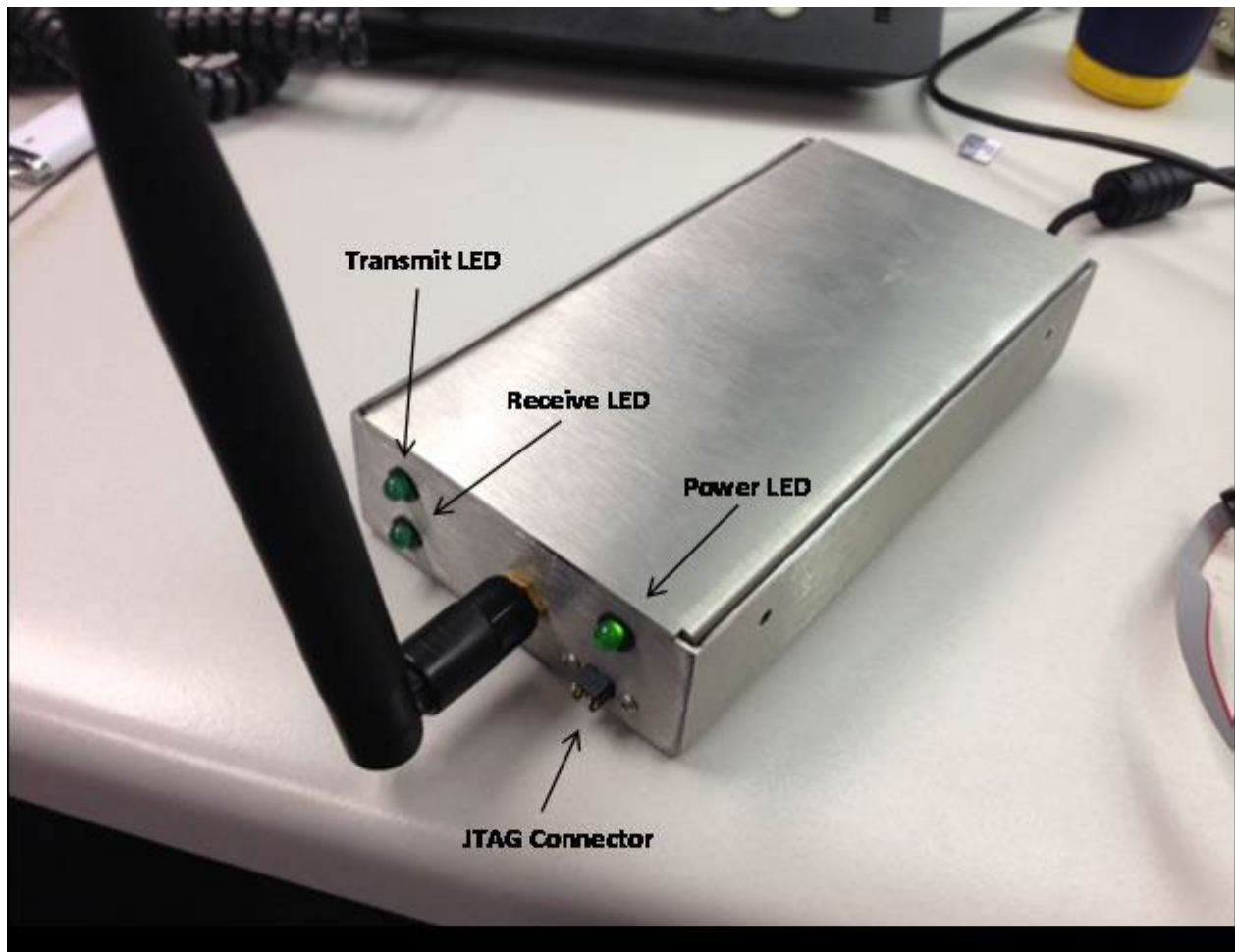
Photo 1: Module with External Antenna
