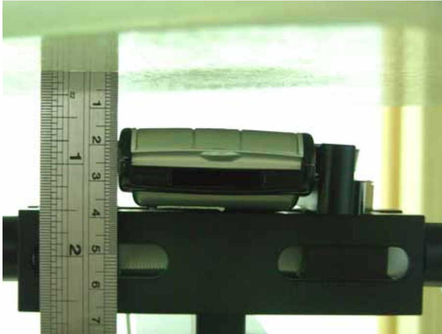
Fig. 9.1 Keypad Up with 1.5cm Gap
