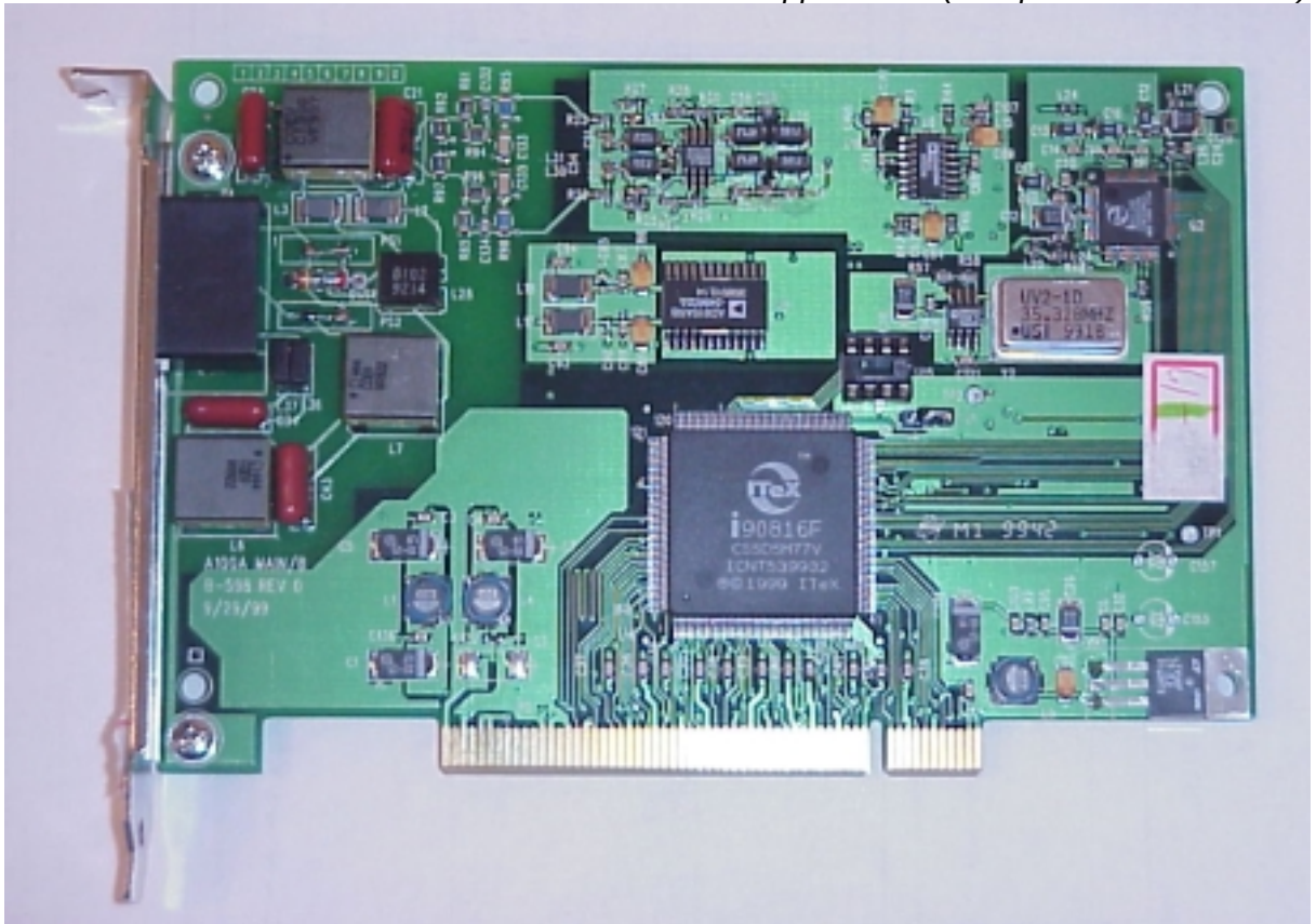
Photos 1 General Appearance (Component Side of EUT)
