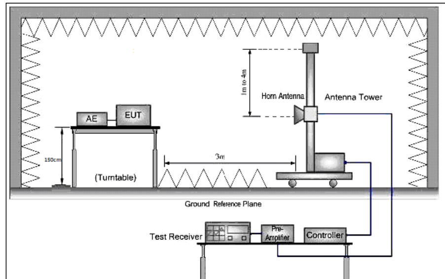
Figure 3. Above 1 GHz
