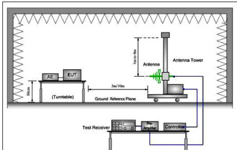
Figure 2. 30MHz to 1GHz
