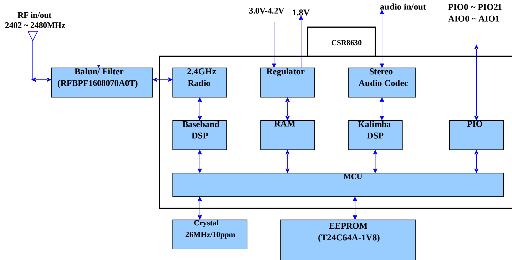
Block Diagram
