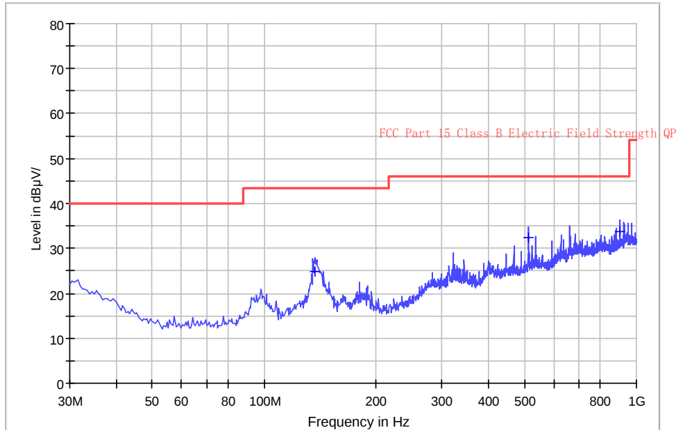
Graphic 1 Radiated Emissions
