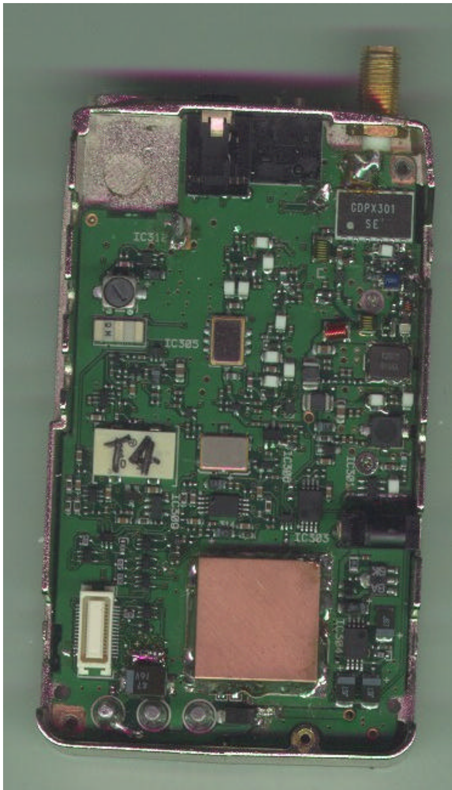
FIGURE 17: Main Board without copper shield
