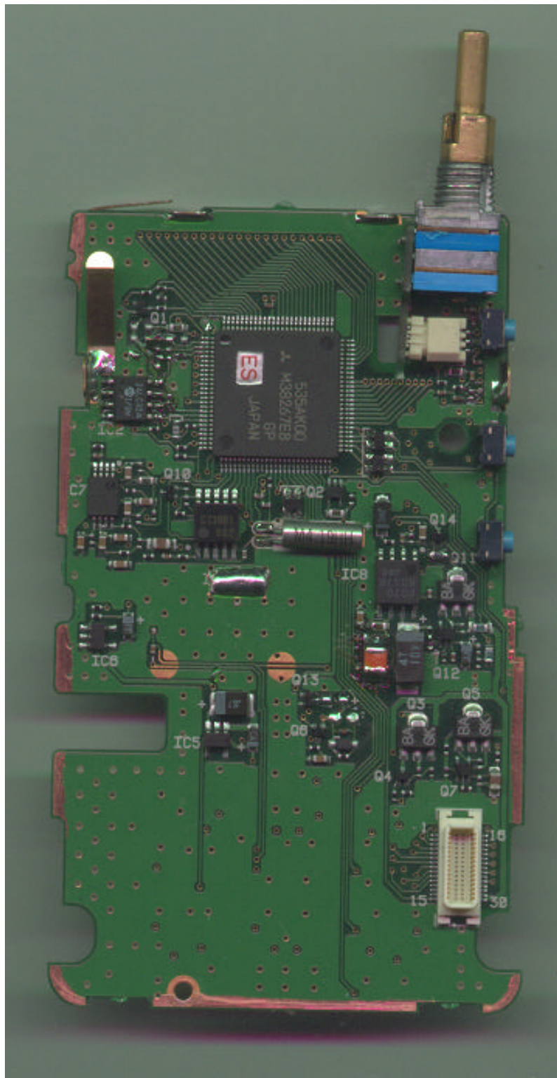
FIGURE 19: Bottom of CPU Board
