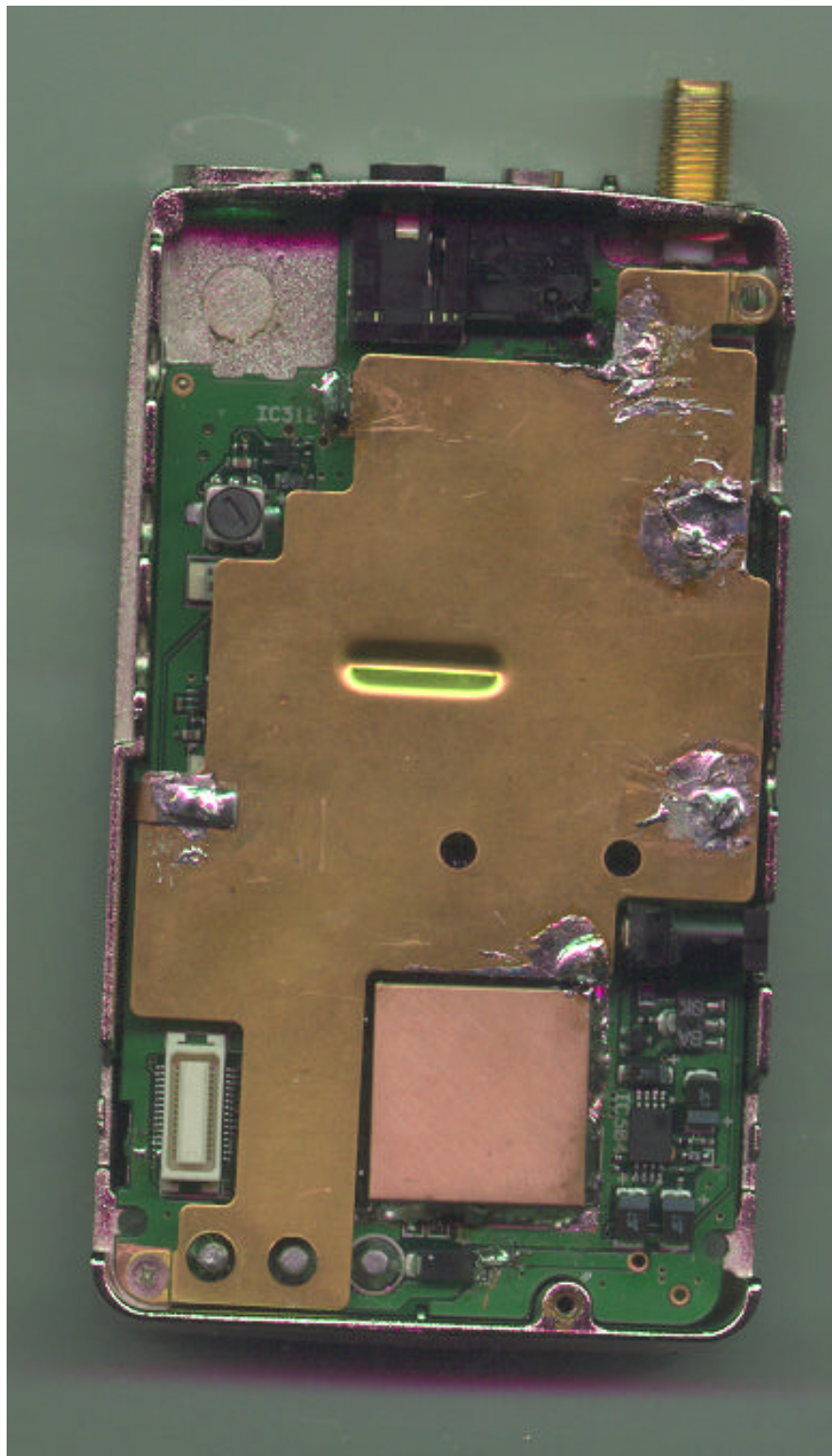
FIGURE 16: Main Board with copper shield
