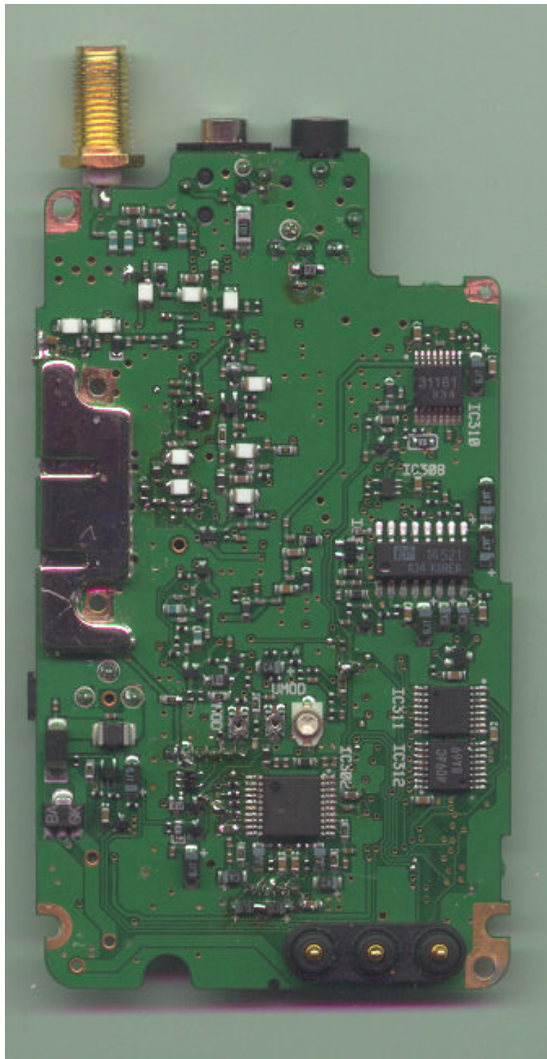
FIGURE 21: Bottom of Main Board
