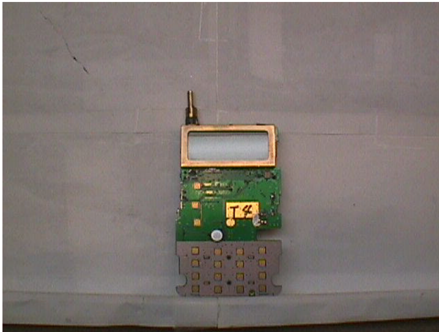
FIGURE 14: Top of CPU board (LCD Side)
