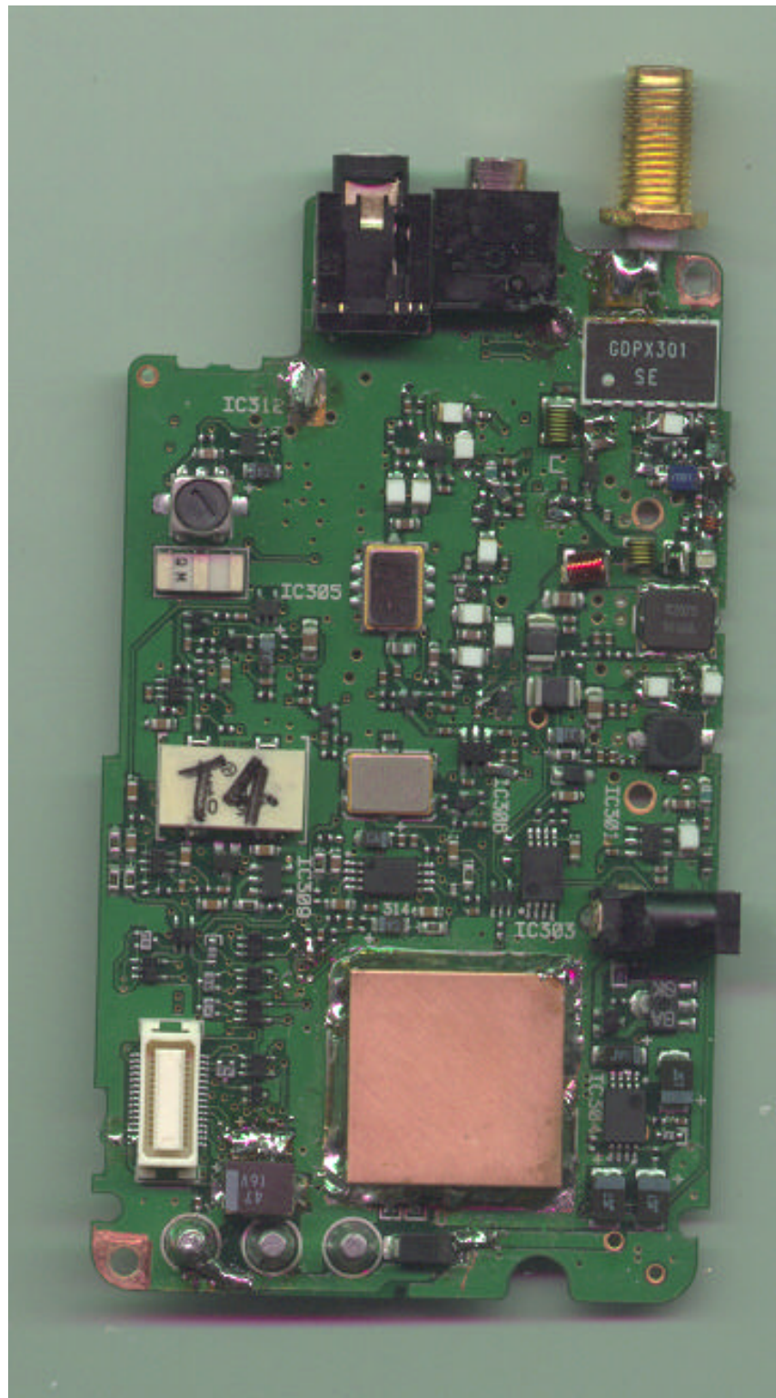
FIGURE 22: Top of Main Board
