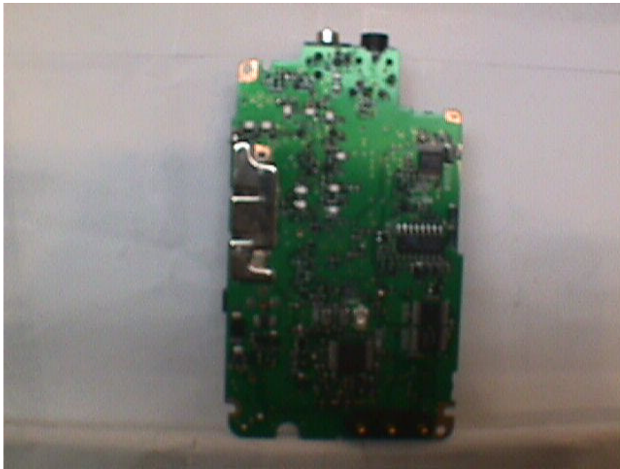
FIGURE 19: Bottom of Main Board
