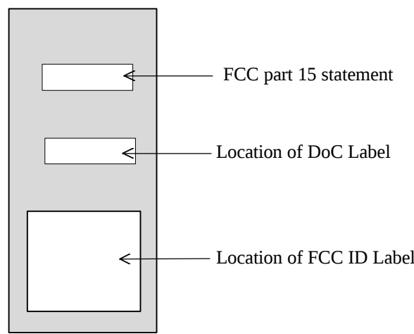
FIGURE 2: LOCATION OF LABELS ON EUT
