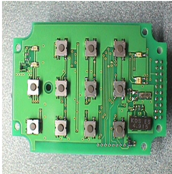
TOP VIEW OF KEYPAD PCB
