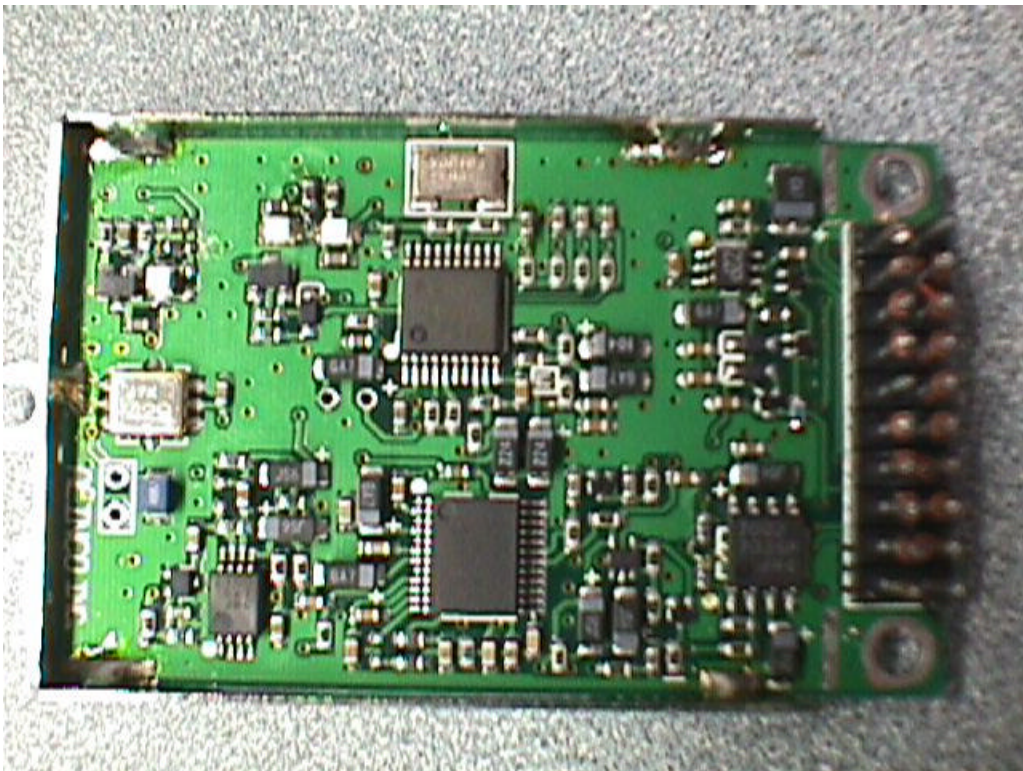
BOTTOM VIEW OF RF PCB
