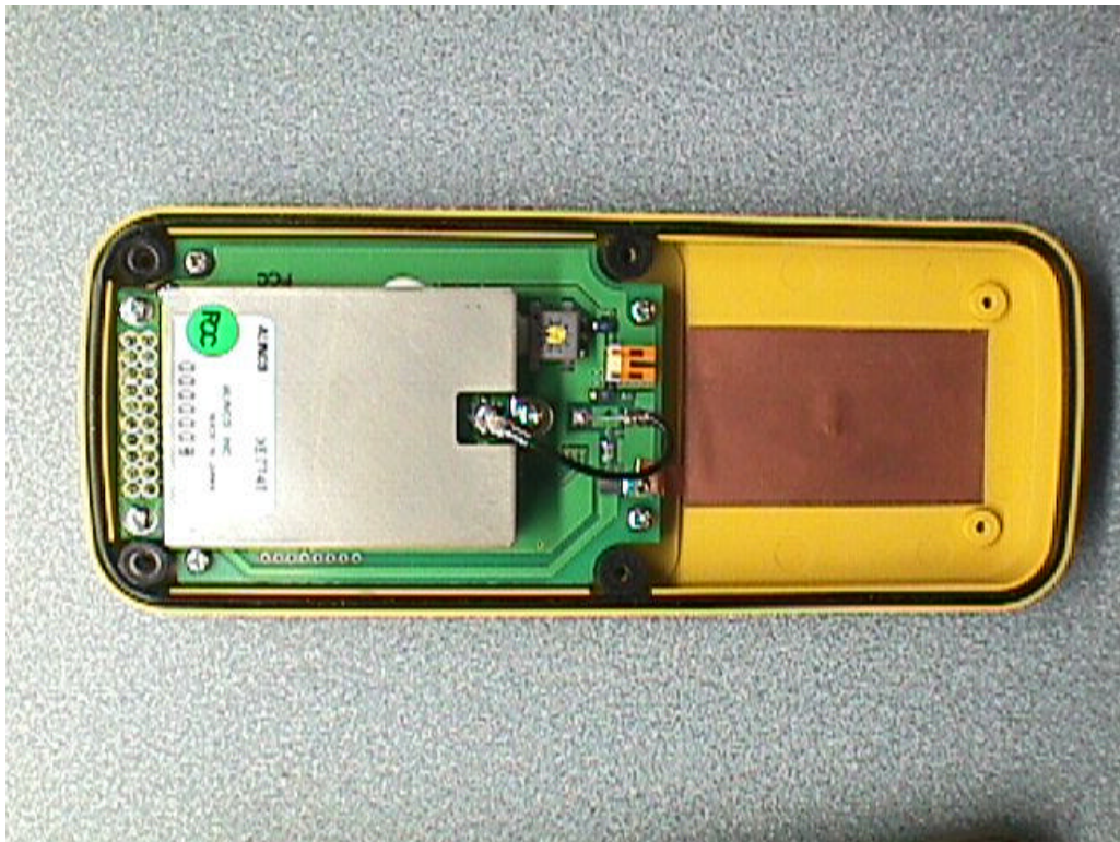
INSIDE VIEW OF KEYPAD AND RF ASSEMBLY TOP COVER
