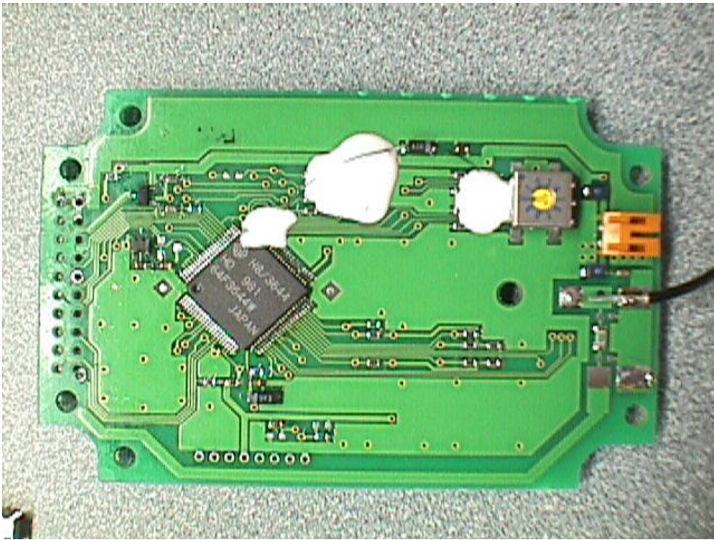
BOTTOM VIEW OF KEYPAD PCB
