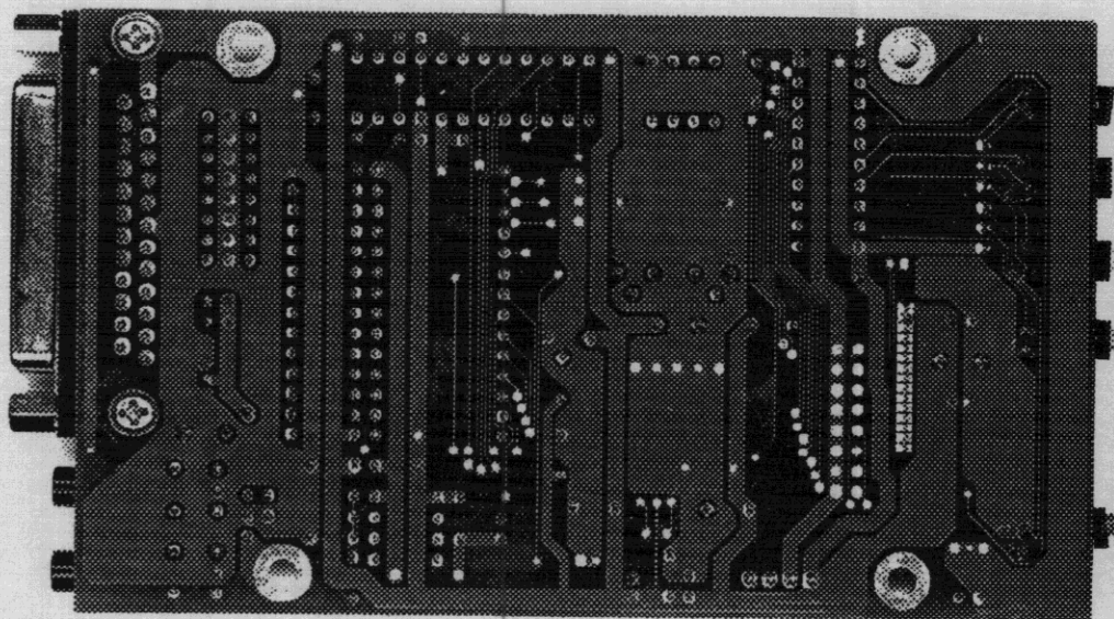
Figure 21: DSSNet Auxiliary Board, Solder Side
