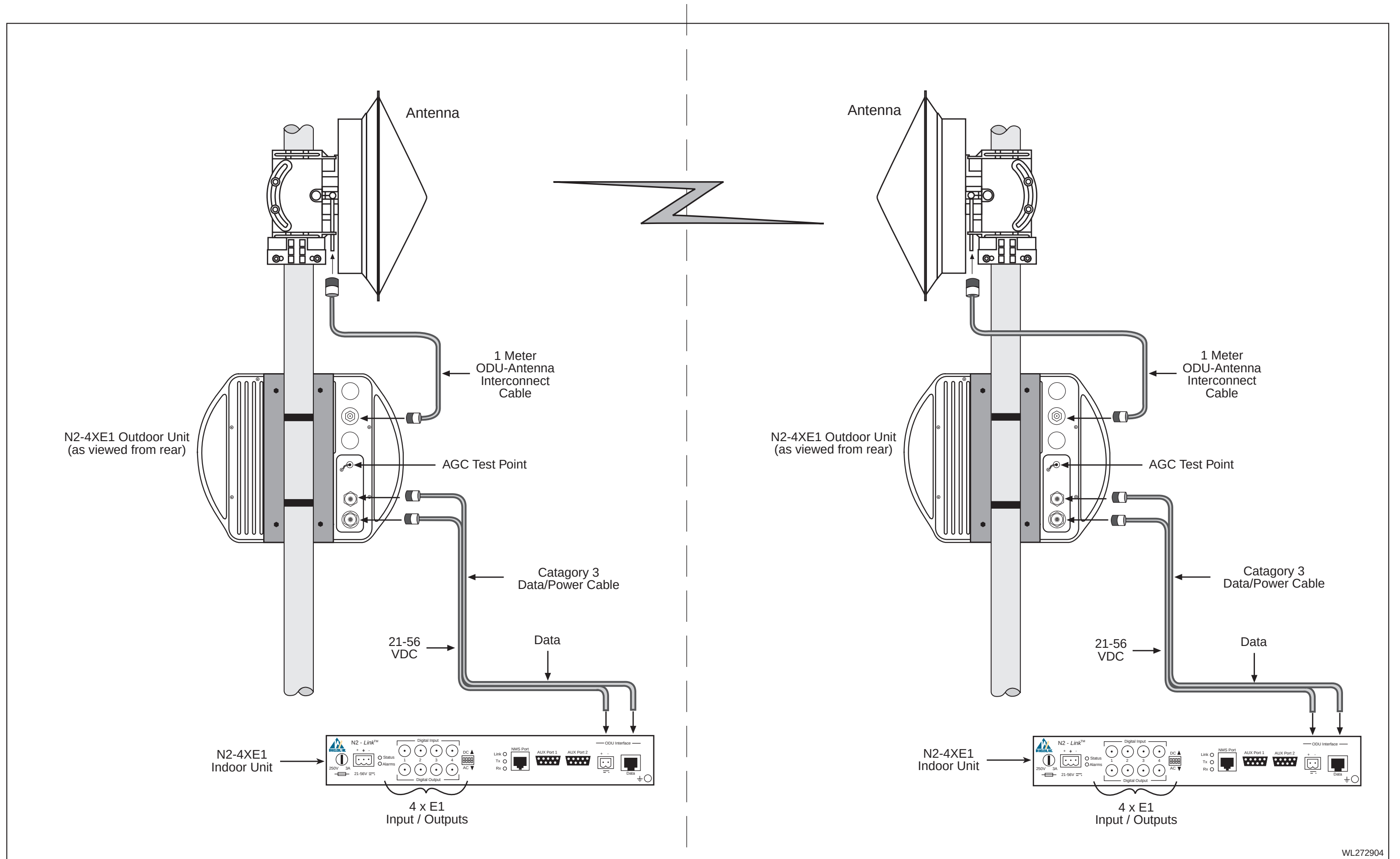
Figure 2.1 - Typical Deployment of a N2-4XE1 Link in a Point-to-Point Configuration
