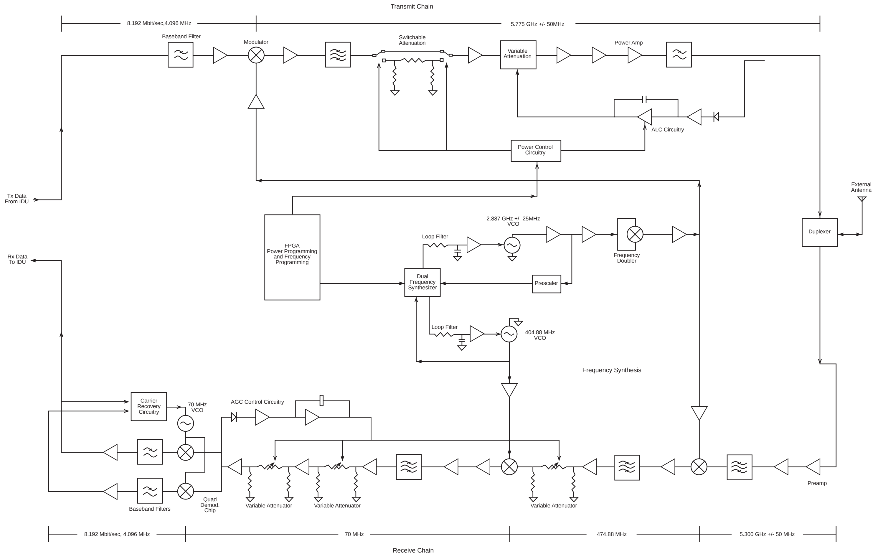
Figure 2.4 - N2-4XE1 Block Diagram
