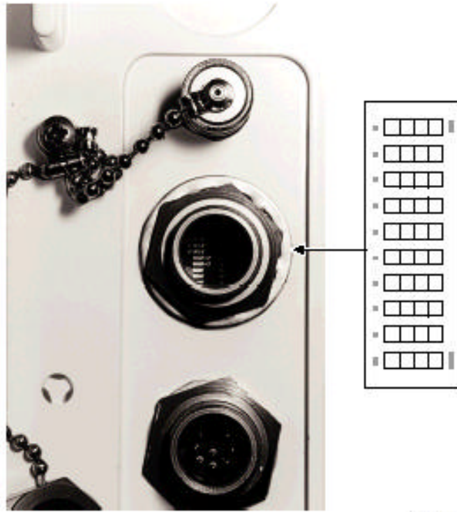
Figure 3.8 - DIP Switch Access and Configuration Information
