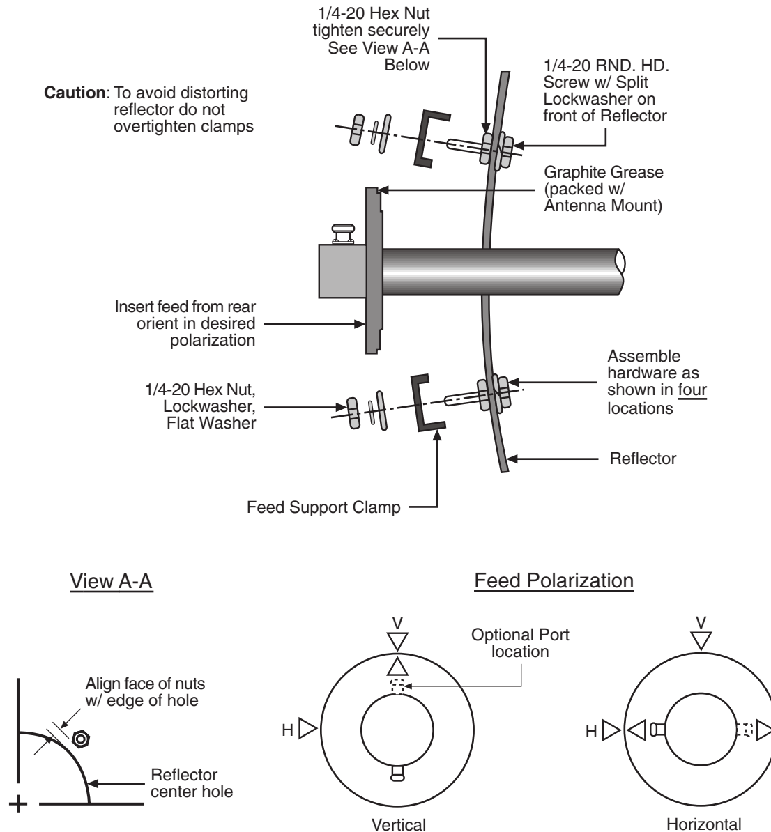
Figure 4.15 - Feed Horn Installation
