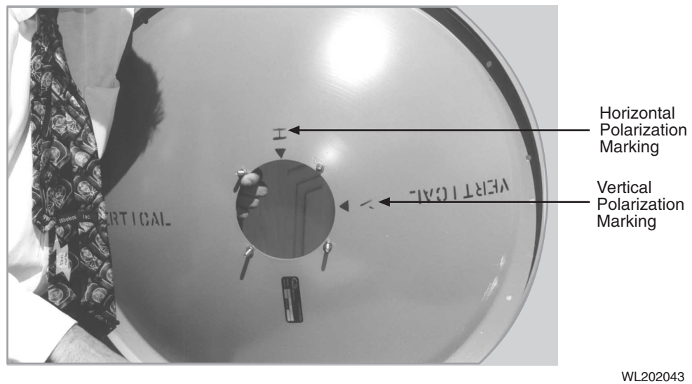
Figure 4.17 - Parabola Rear View Showing Polarization Reference Markings
