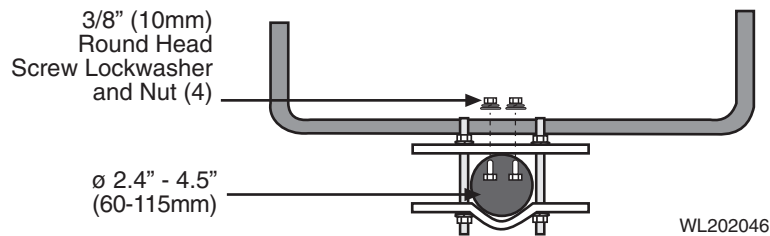
Figure 4.20 - Azimuth Clamp/Shear Stop Assembly
