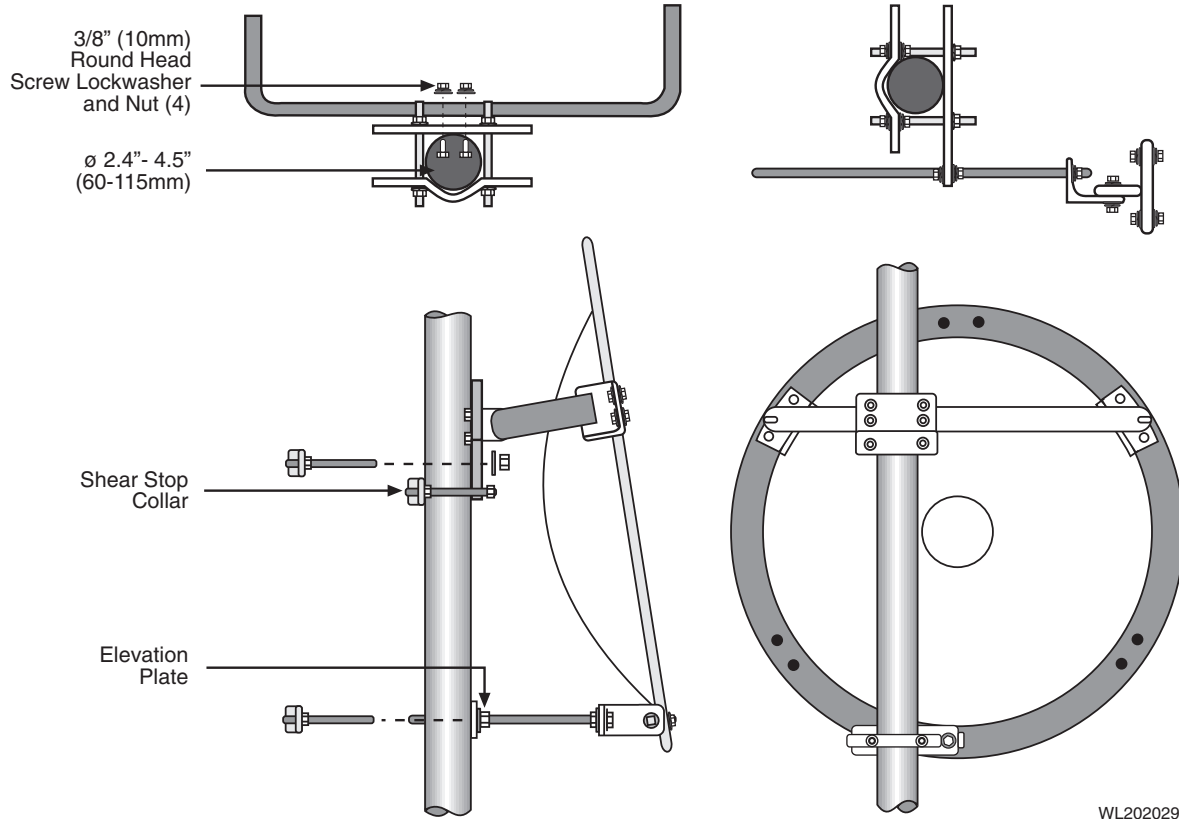
Figure 4.7 - Mount Configuration
