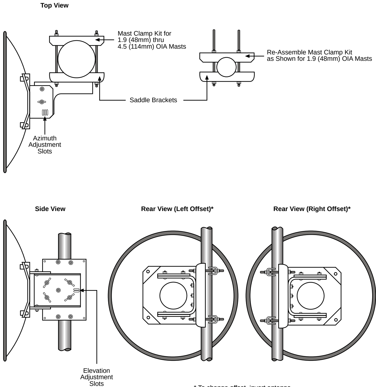
Figure C.2 - Mount Configuration
