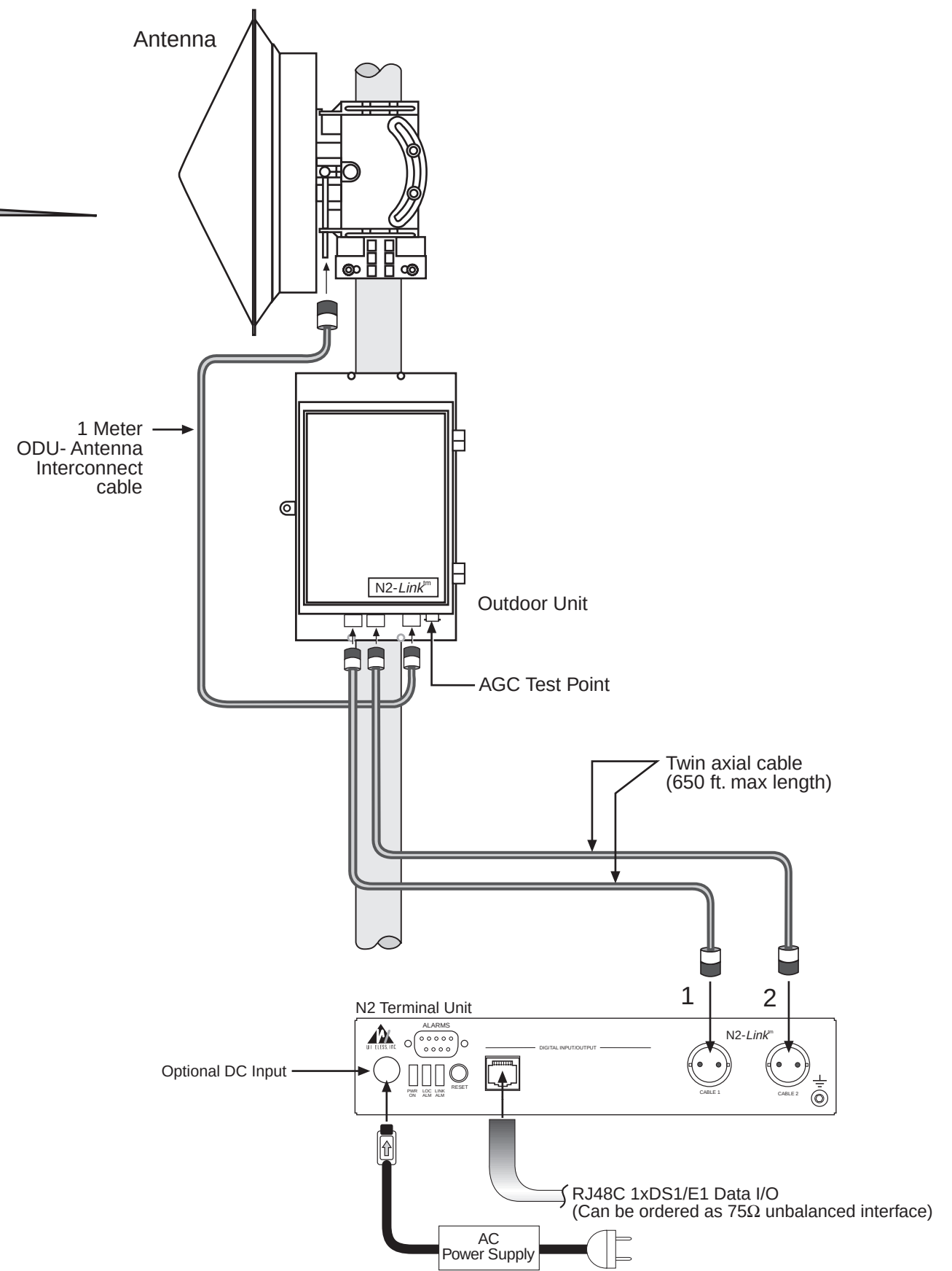
Figure 2.1 - Typical Deployment of a N2-Link in a Point-to-Point Configuration
