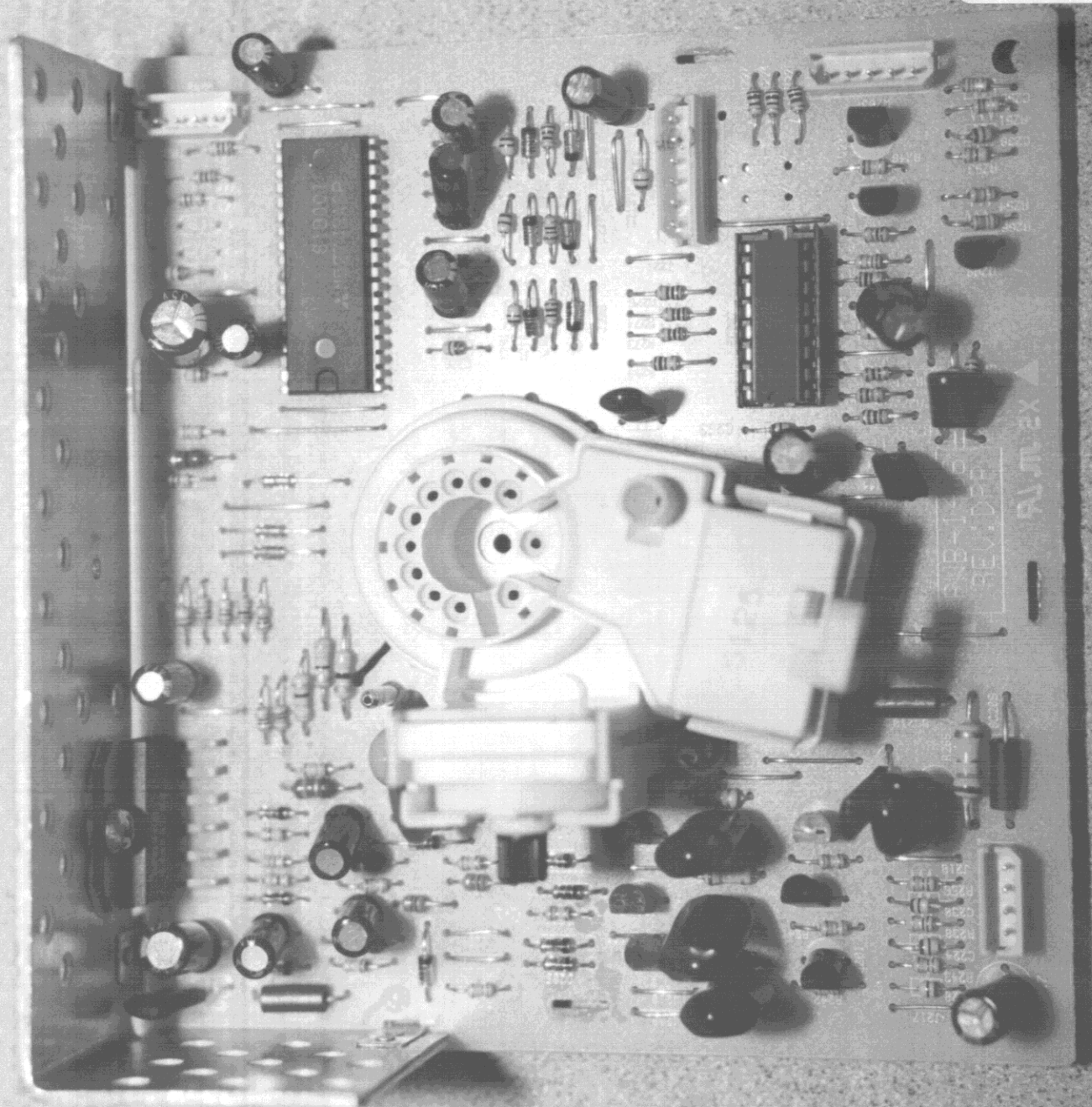
FIGURE 12 NECK OF PCB COMPONENT SIDE PAGE 29 WORK ORDER NUMBER 980539 KD-1511T 15" MONITOR
