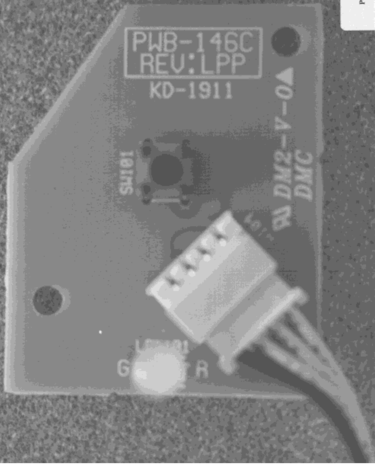
Figure 21: Power Switch/LED Board, Component Side
