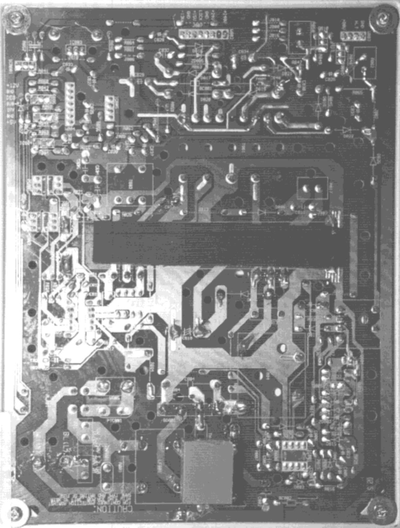
Figure 17 Solder View of Left Side Circuitry
