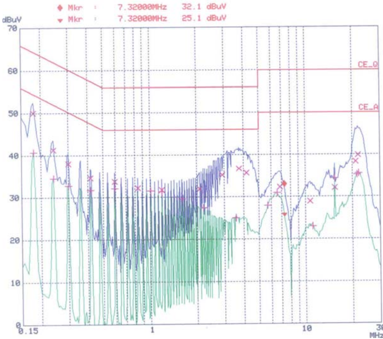
< Neutral line >
