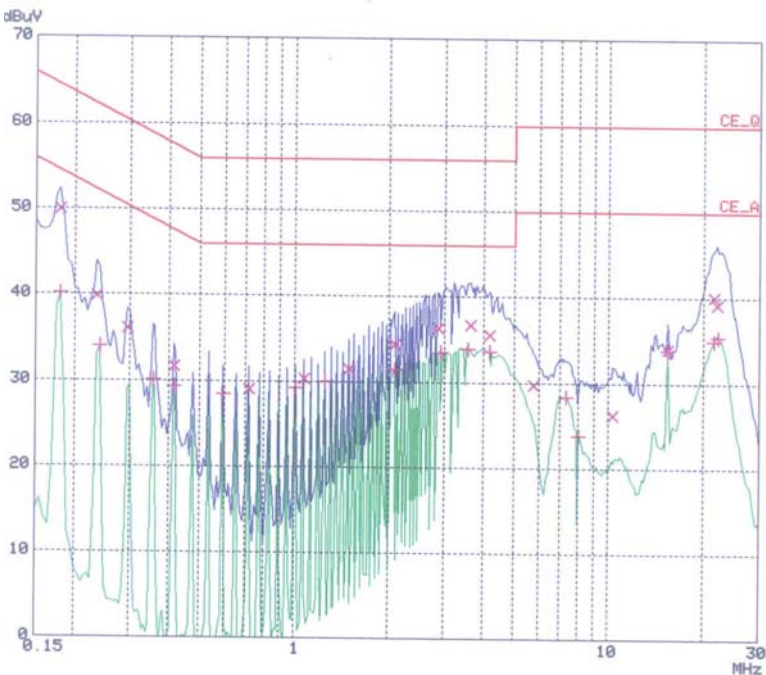
< Hot line >
