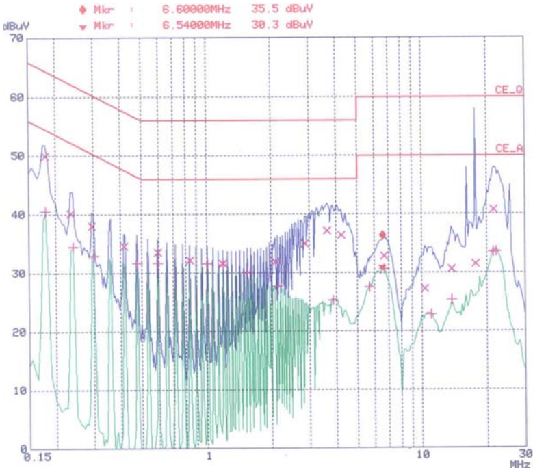
< Neutral line >
