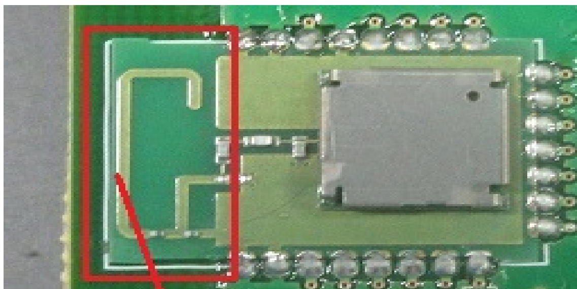
Antenna 1
