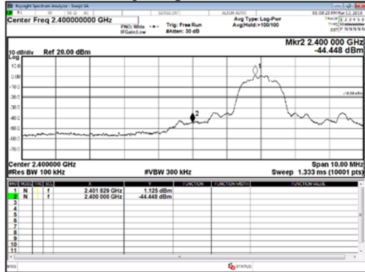
Single hop 2402 MHz
