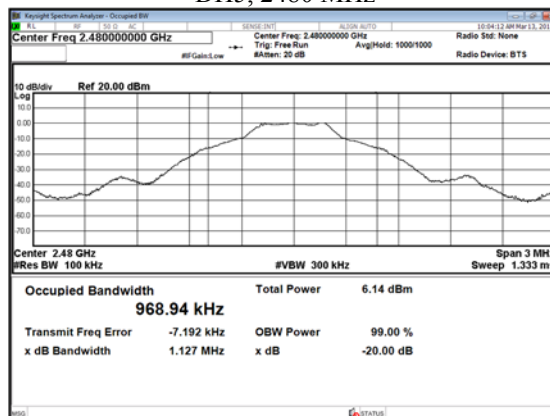
DH5, 2480 MHz
