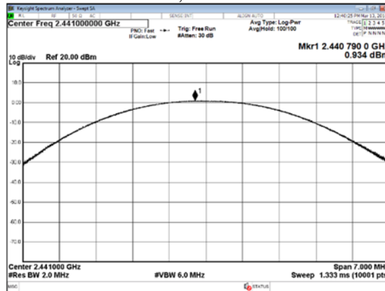
2DH5, 2441 MHz
