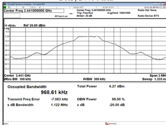
DH5, 2441 MHz
