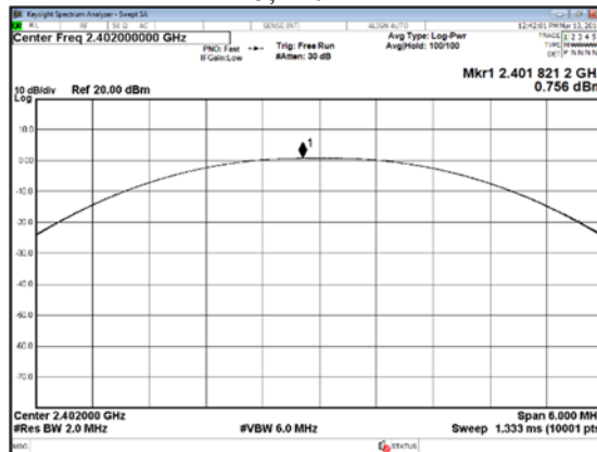
DH5, 2402 MHz
