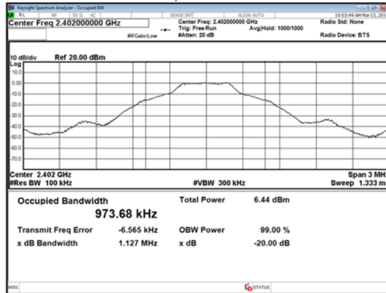
DH5, 2402 MHz
