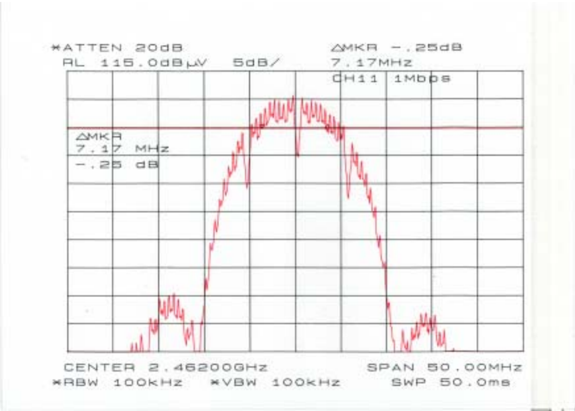
Chart of ch 11 with 1 Mbps
