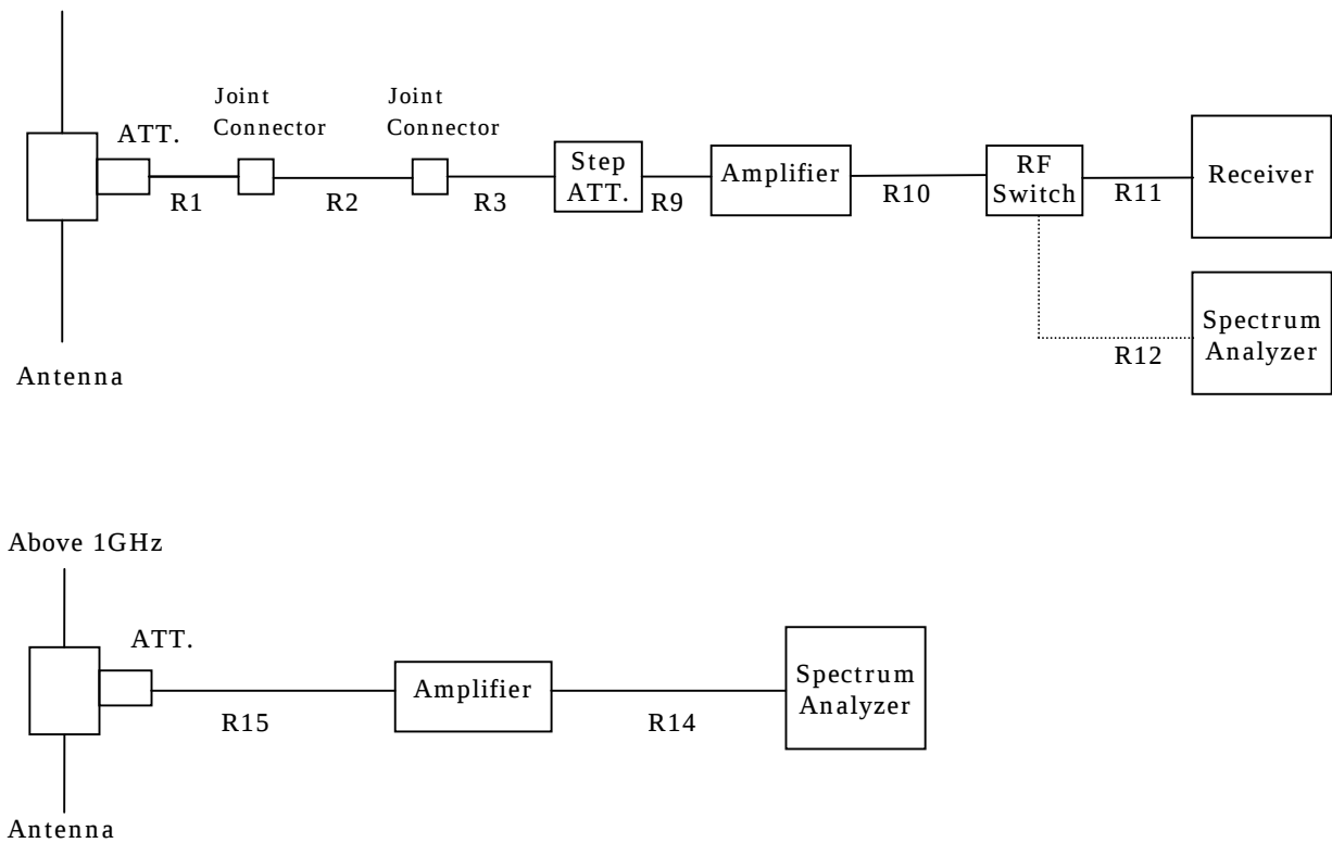
Schema for the radiated electric field measurement
