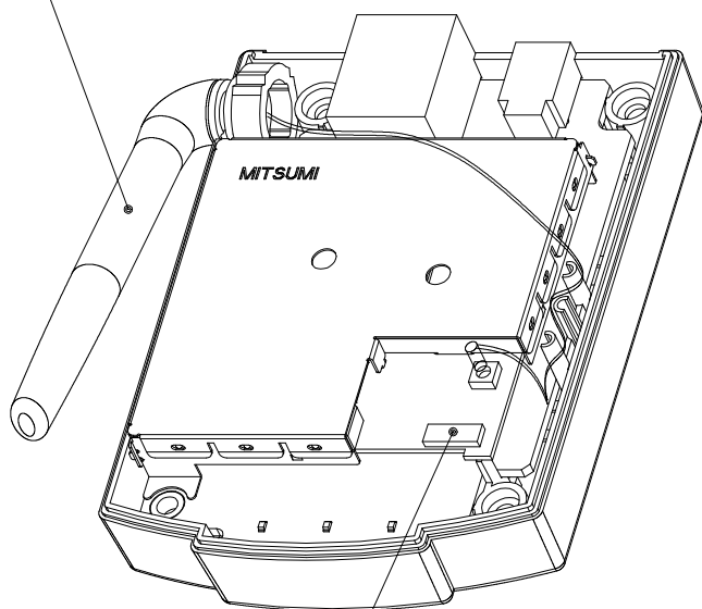
SLEEVE ANTENNA (for TX/RX)
