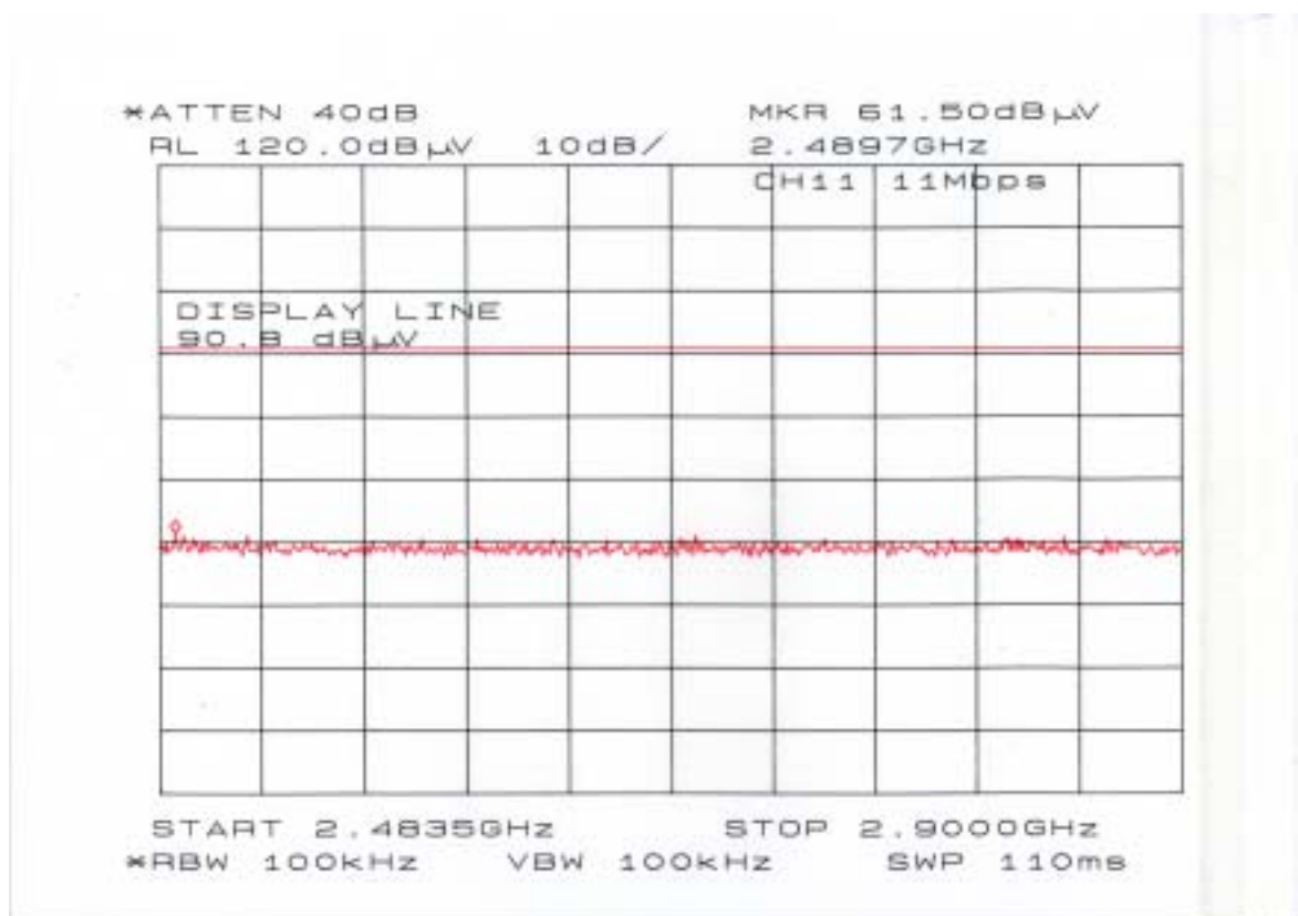
Chart of ch 11 with 11Mbps (2.4835GHz-2.9GHz)
