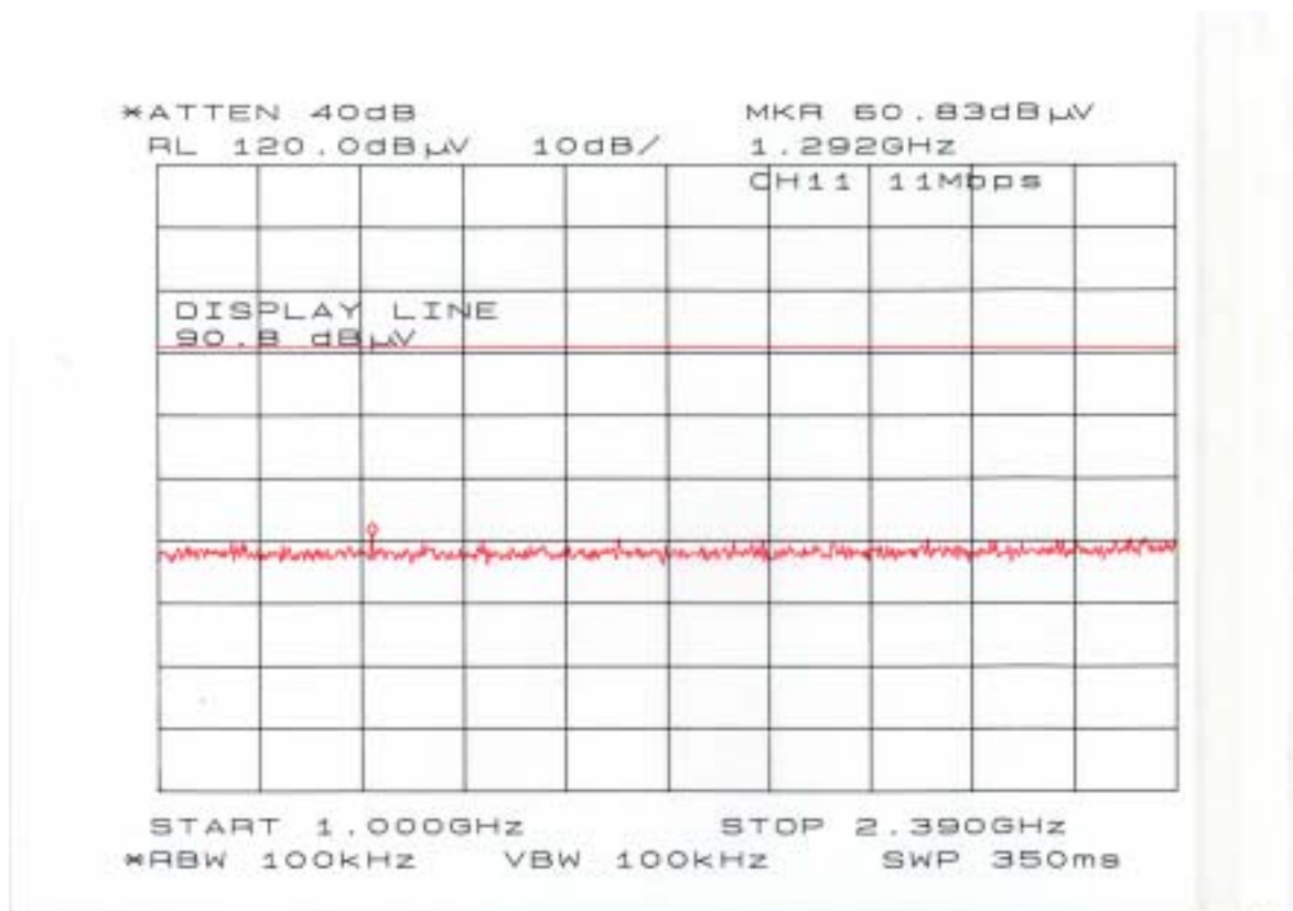
Chart of ch 11 with 11Mbps (1GHz-2.39GHz)
