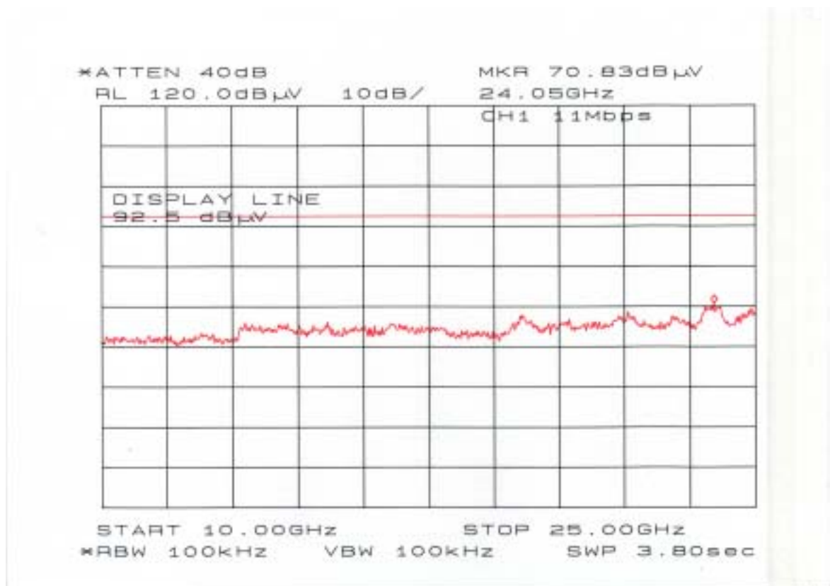
Chart of ch 1 with 11Mbps (10GHz-25GHz)
