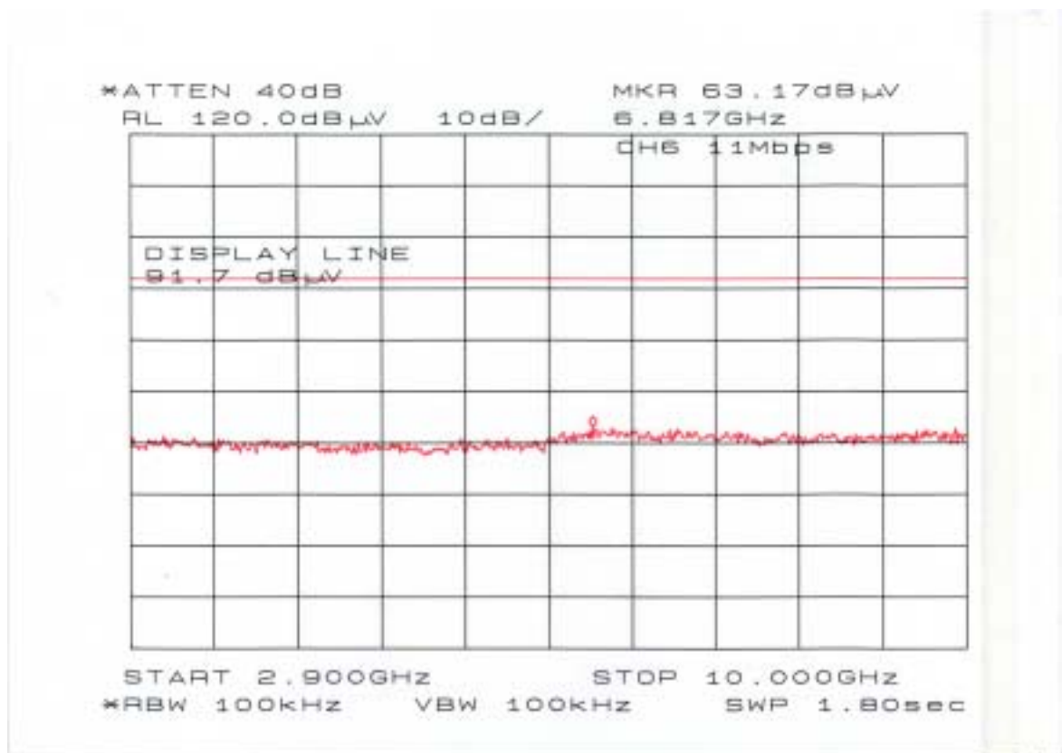
Chart of ch 6 with 11Mbps (2.9GHz-10GHz)
