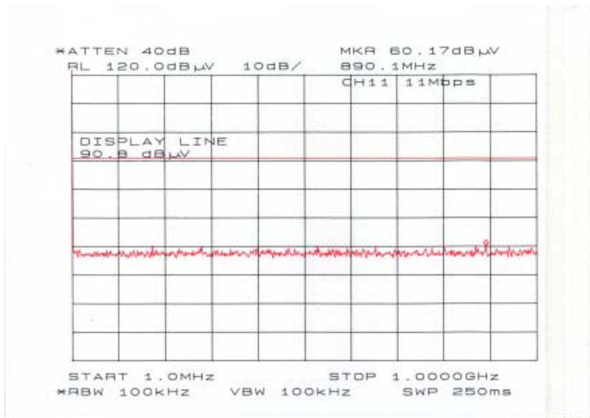
Chart of ch 11 with 11Mbps (1MHz-1GHz)
