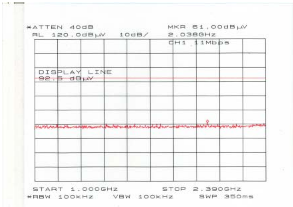
Chart of ch 1 with 11Mbps (1GHz-2.39GHz)
