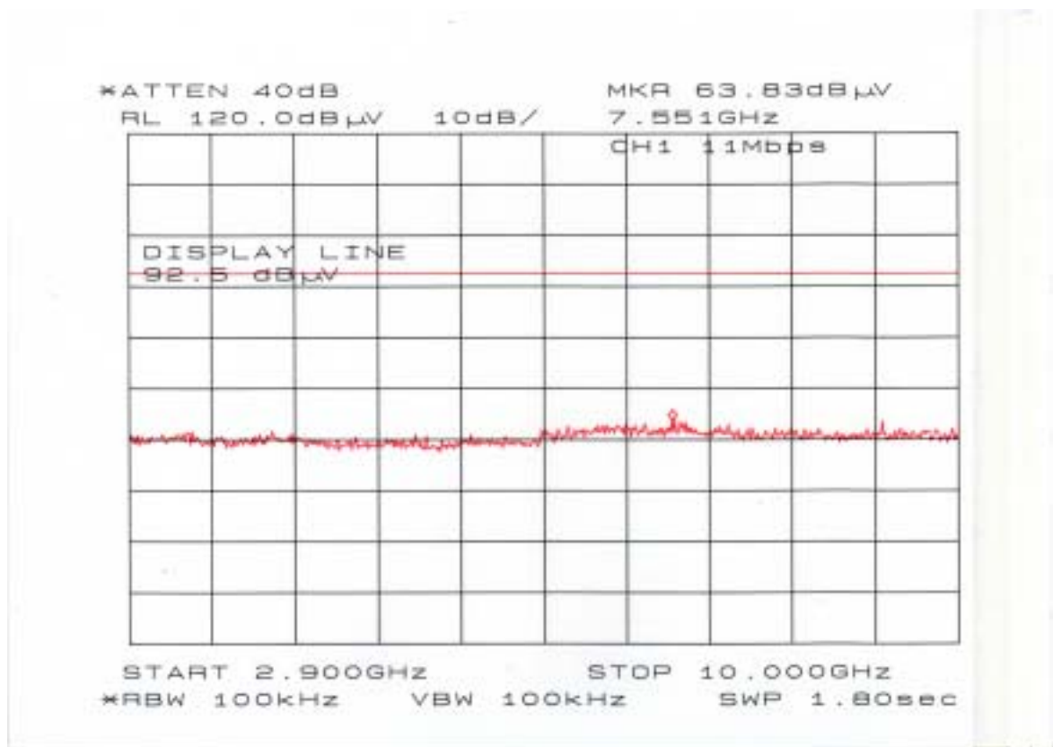
Chart of ch 1 with 11Mbps (2.9GHz-10GHz)
