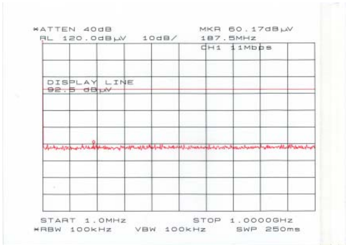
Chart of ch 1 with 11Mbps (1MHz-1GHz)
