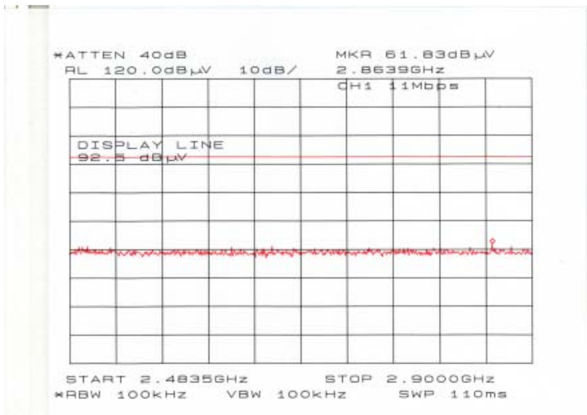
Chart of ch 1 with 11Mbps (2.4835GHz-2.9GHz)
