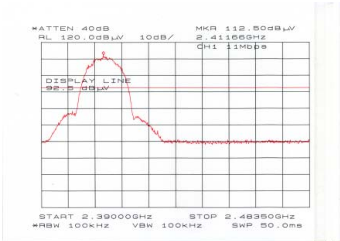
Chart of ch 1 with 11Mbps (2.39GHz-2.4835GHz)
