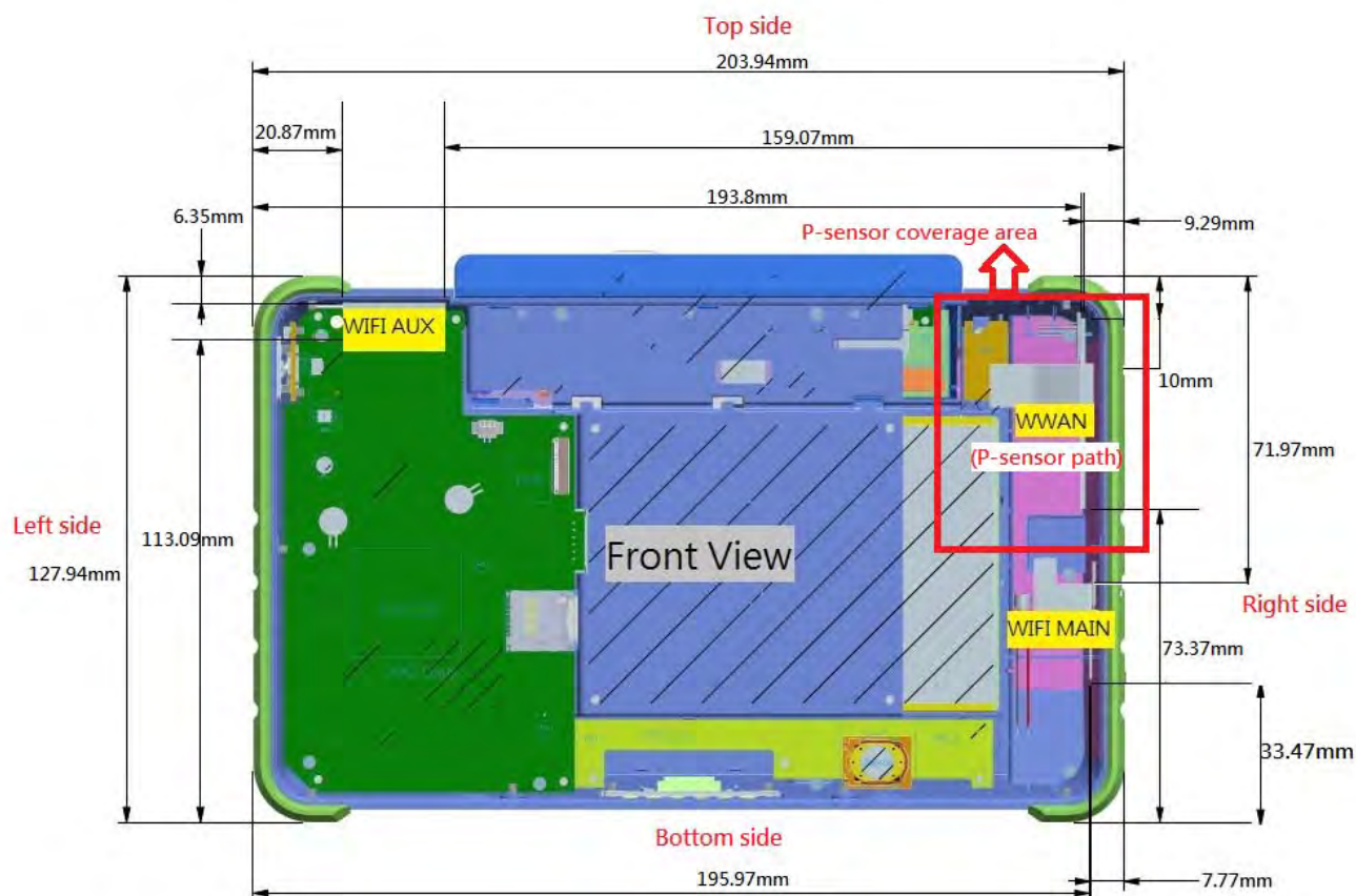
Fig.10 Antenna position of EUT (Front view)
