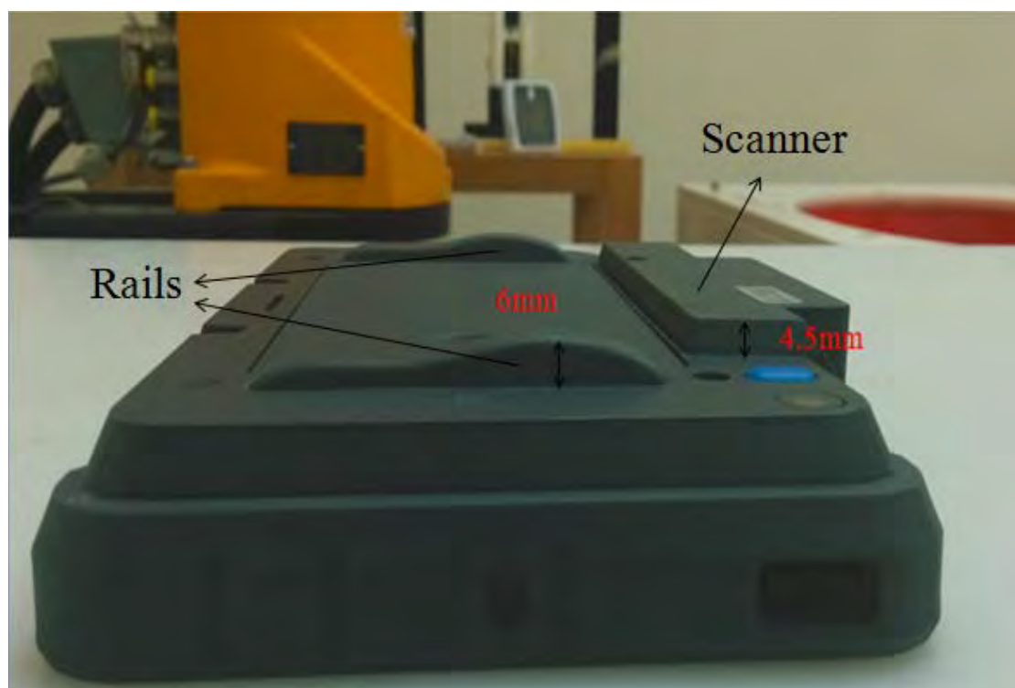
Fig.9 Side view of EUT(with scanner and rails)
