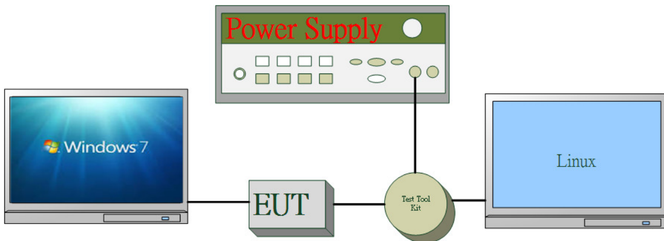
Fig. 2-1 Radiated Emission & Conducted (Antenna Port) Configuration
