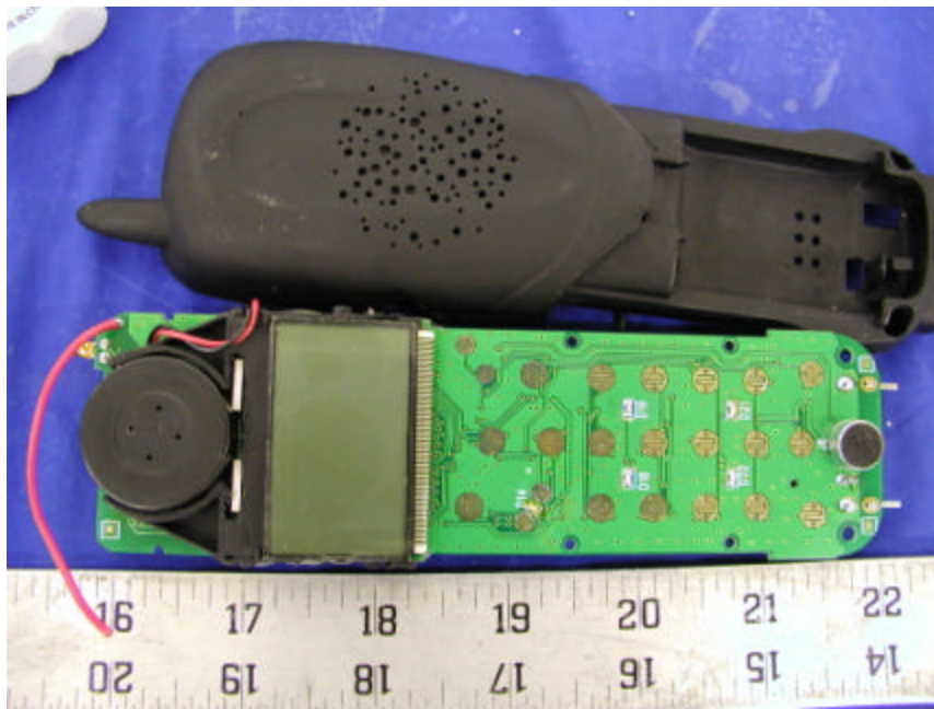
Handset – Main Board Solder View
