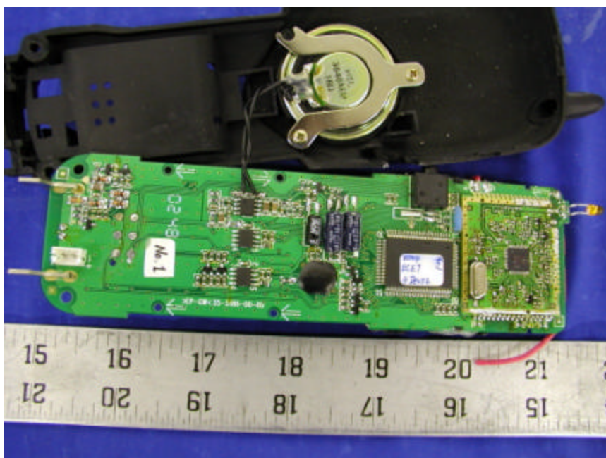
Handset – Main Board Component View
