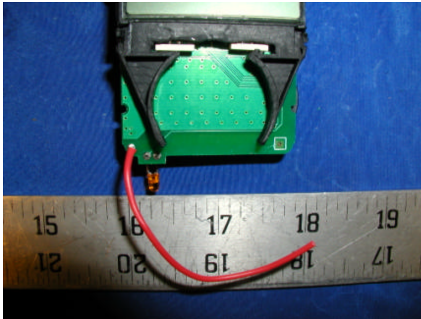
Handset – Transmitter Solder View
