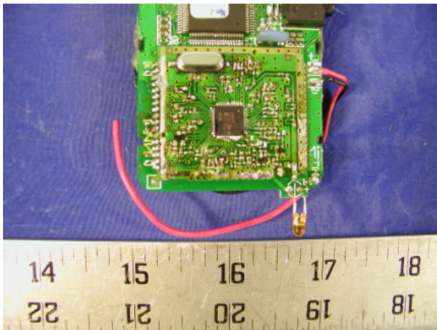
Handset – Transmitter Component View
