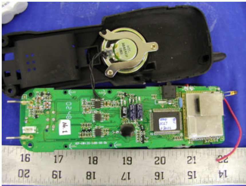
Handset – Main Board Component View with subshield
