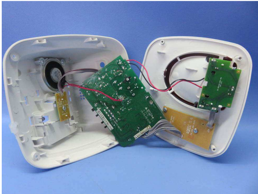
Base Unit
