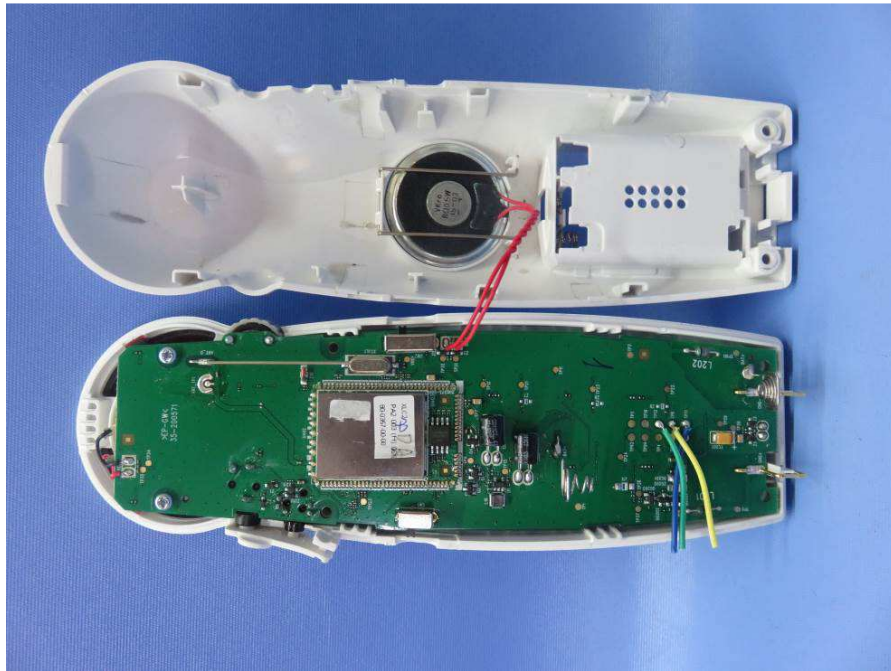
Handset
