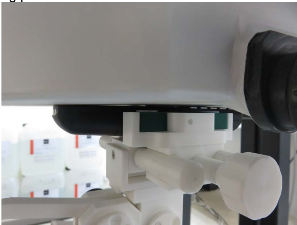
Figure 5 – Front surface with 0mm Separation
