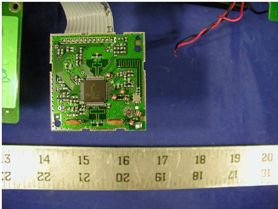
Terminal Transceiver - Component View
