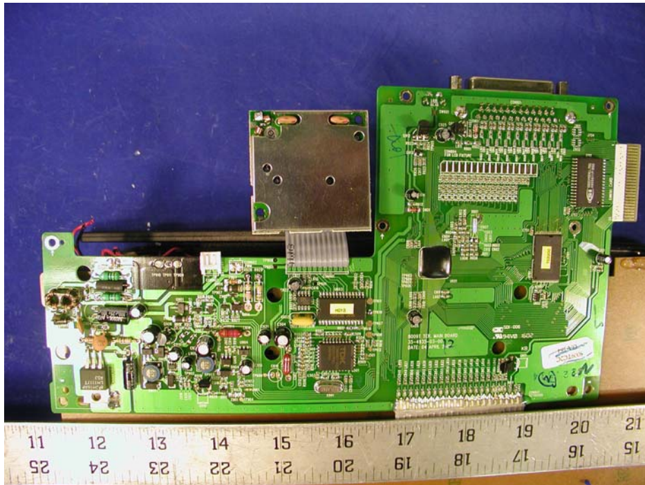
Terminal Main Board - Component View
