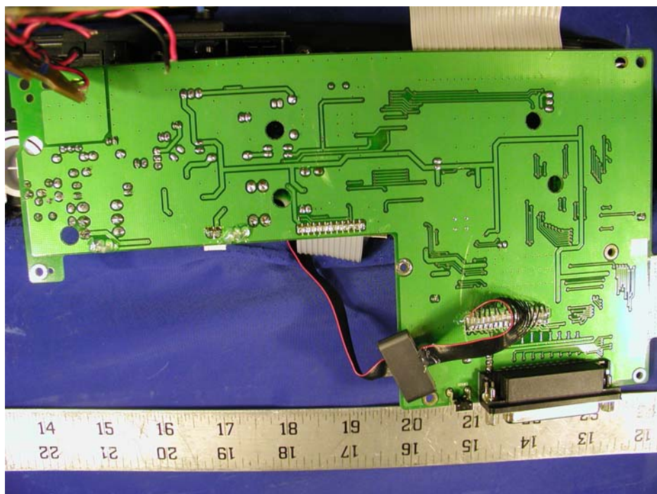
Terminal Main Board - Solder View
