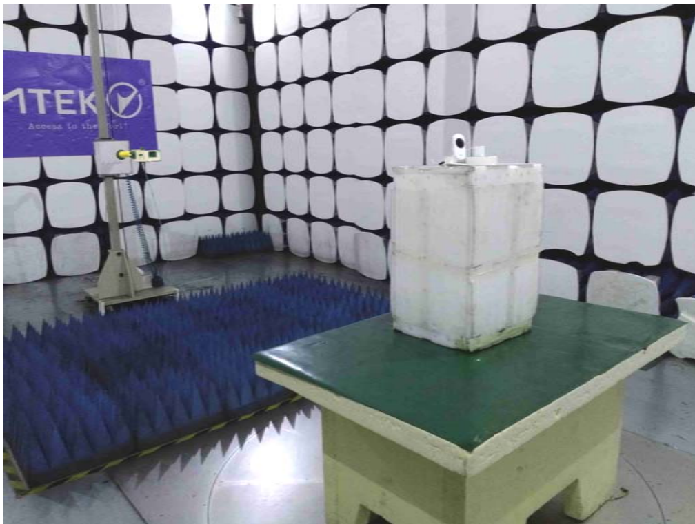
Radiation Emission(18GHz-26.5GHz)
