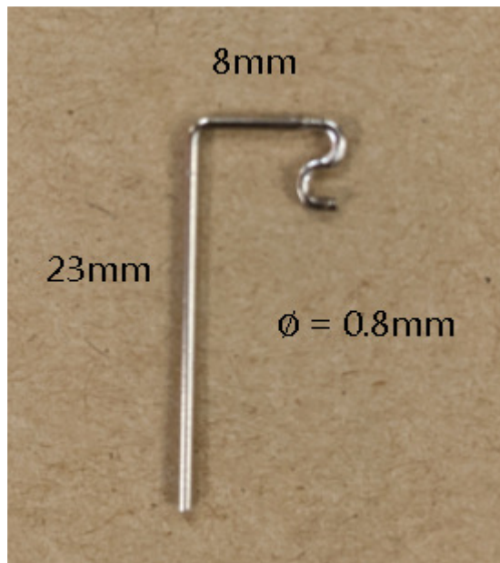
Figure 1 Physical dimension (mm)
