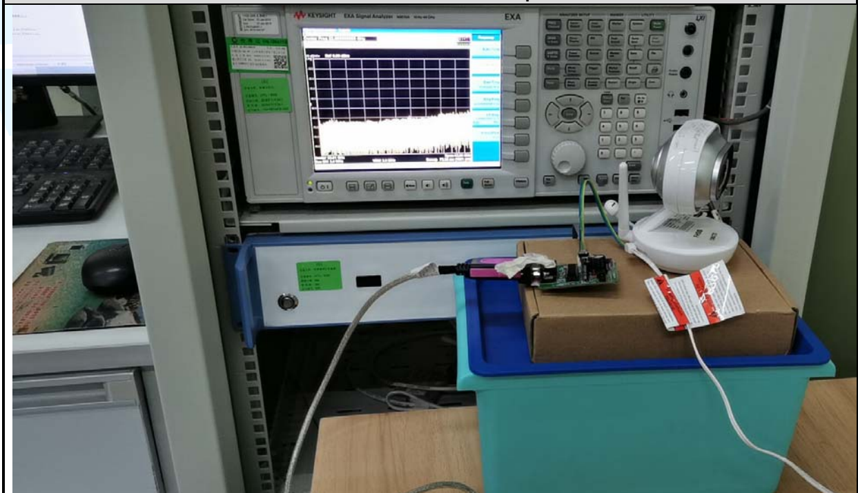
RF Conducted Test Setup
