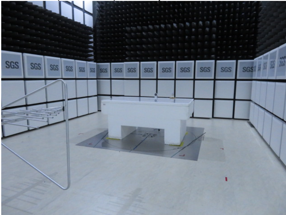
Radiated Emissions (30MHz-1GHz) Test setup
