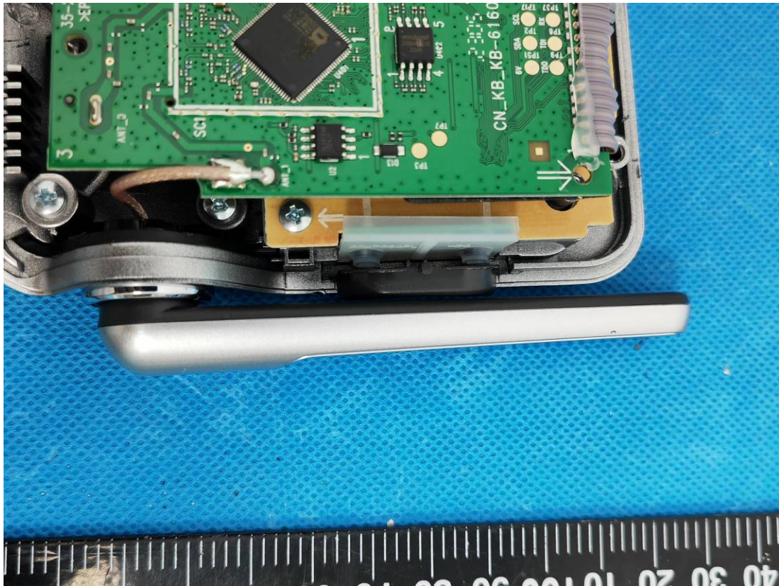
DECT ANT1
