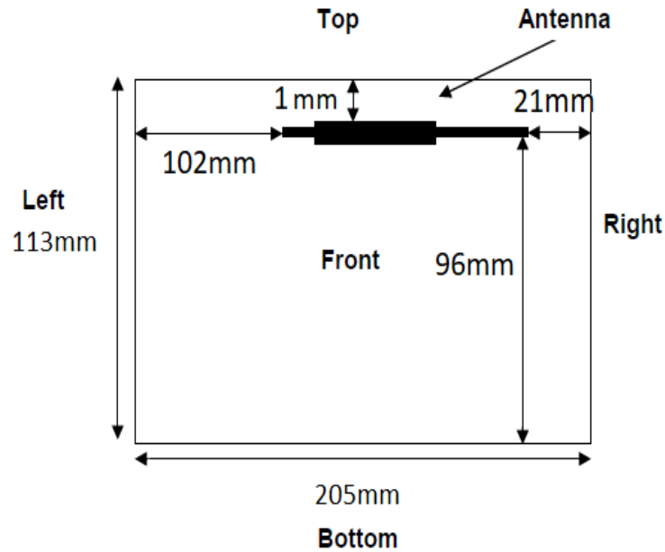
Antenna Closed Configuration
