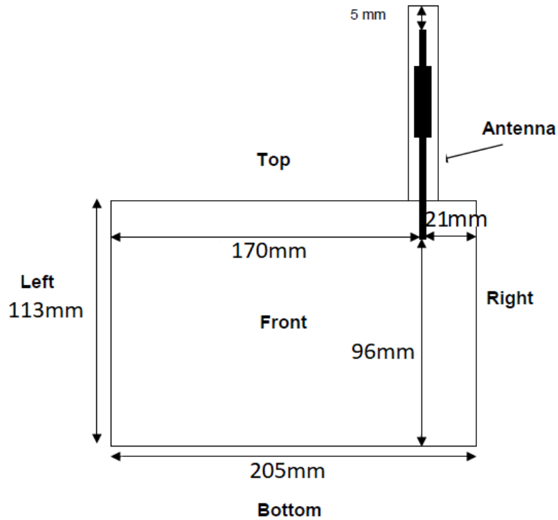
Antenna Extended Configuration
