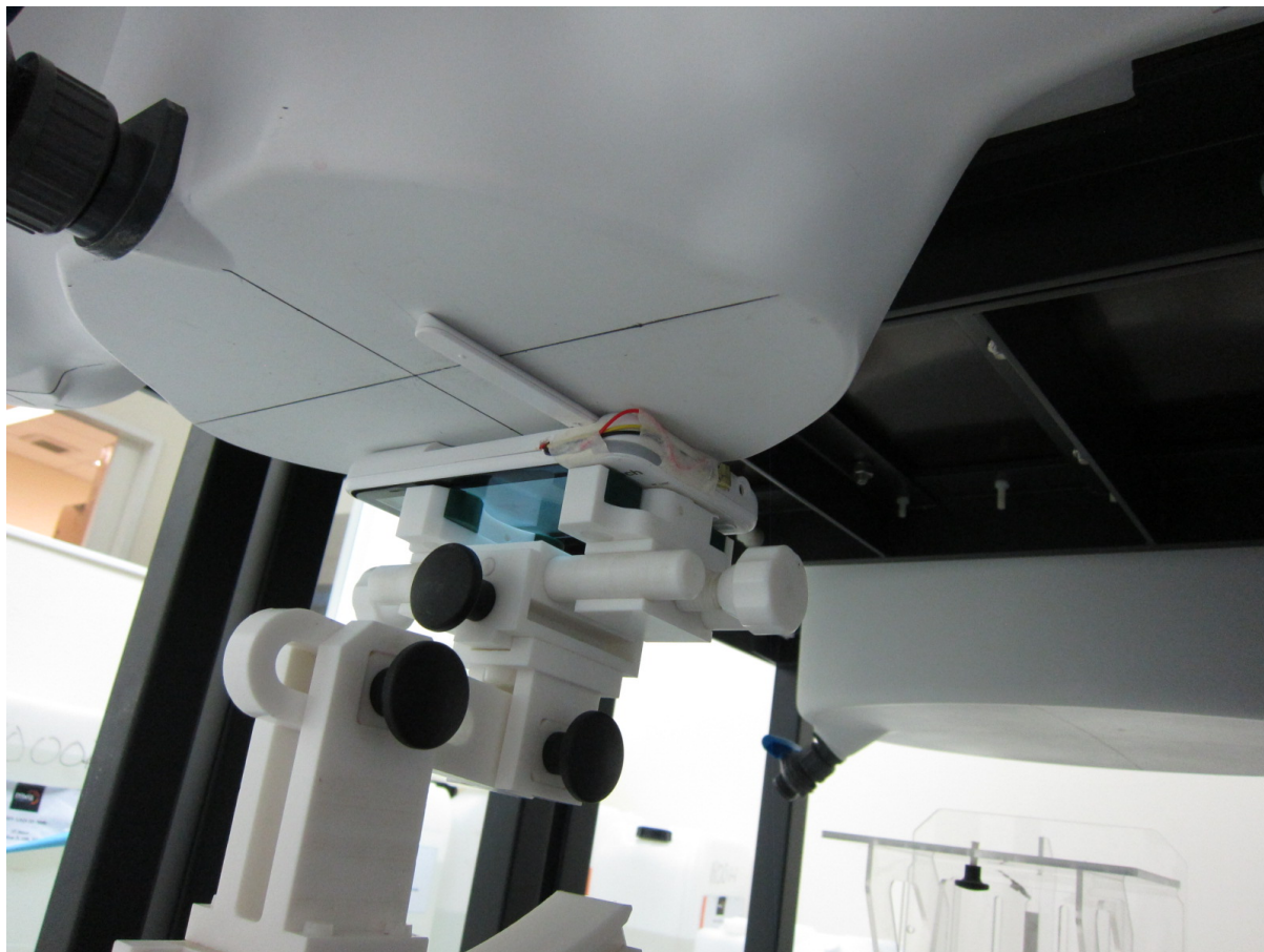
Figure 1 – Back (Antenna extended) with 0mm Separation
