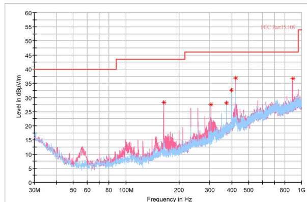
Figure 9. 30M-1GHz
