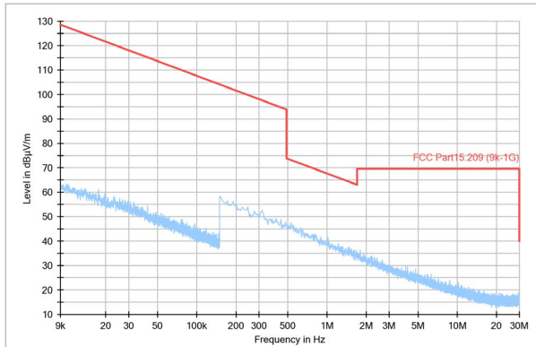
Figure 1. 9k-30MHz
