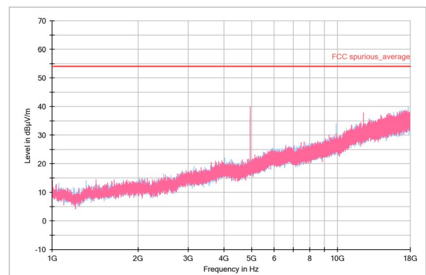
Figure 5. 1-18GHz Average
