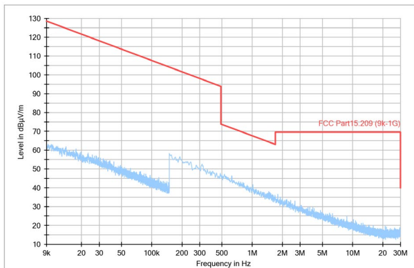
Figure 8. 9k-30MHz
