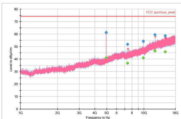
Figure 4. 1-18GHz Peak
