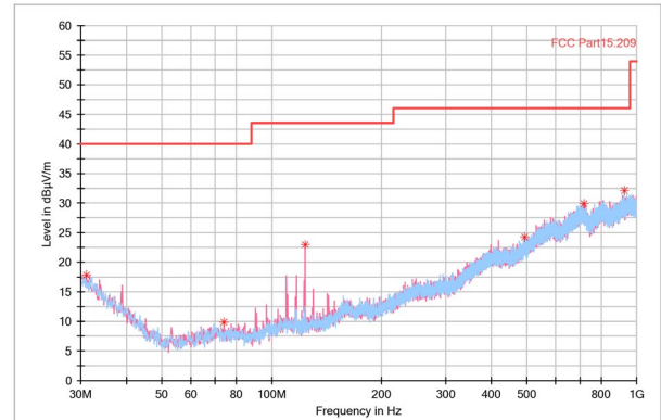
Figure 9. 30M-1GHz
