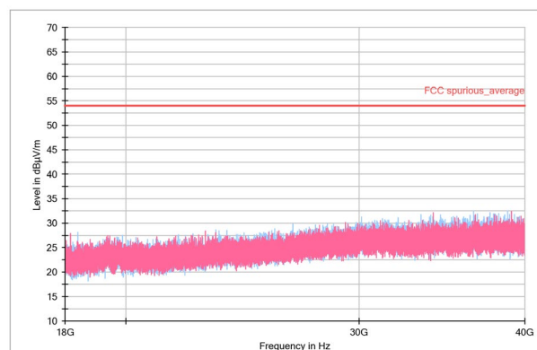
Figure 7. 18-40GHz Average
