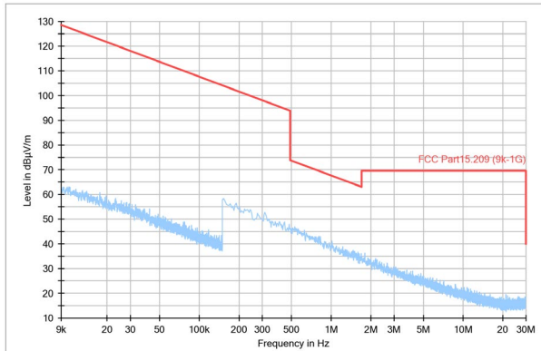
Figure 8. 9k-30MHz
