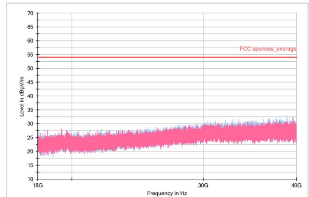
Figure 14. 18-40GHz Average
