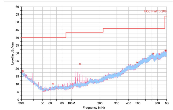
Figure 2. 30M-1GHz
