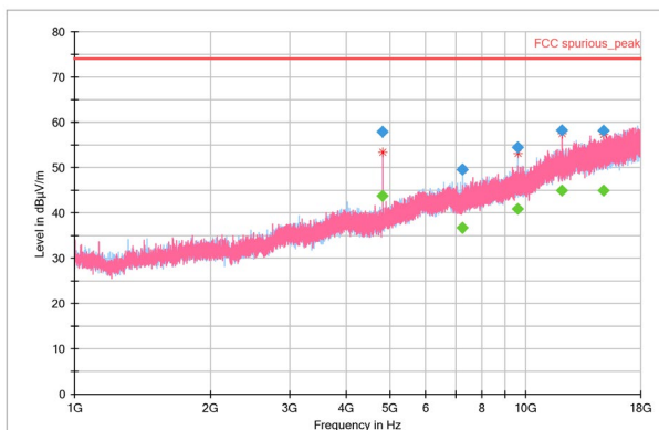
Figure 11. 1-18GHz Peak
