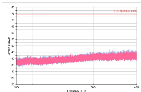
Figure 6. 18-40GHz Peak
