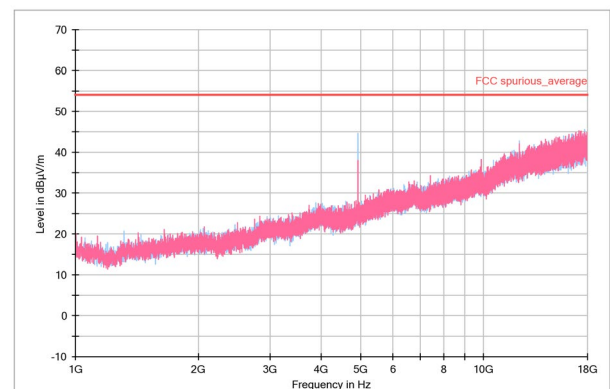
Figure 5. 1-18GHz Average
