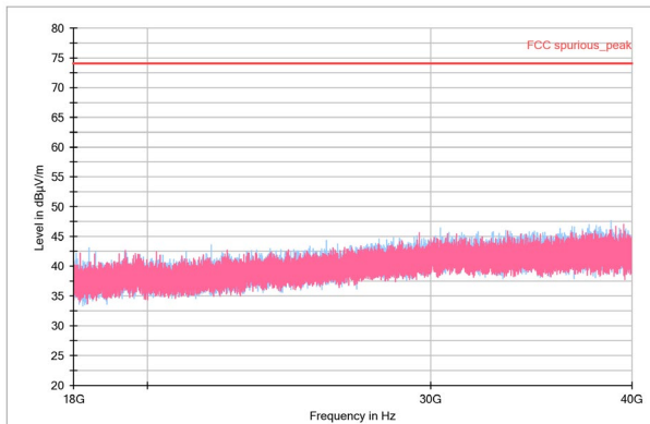
Figure 13. 18-40GHz Peak
