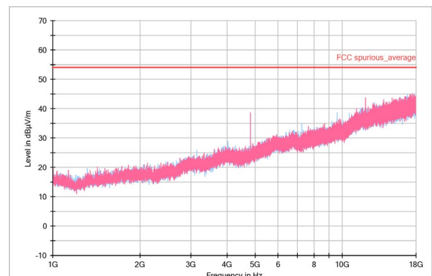
Figure 12. 1-18GHz Average
